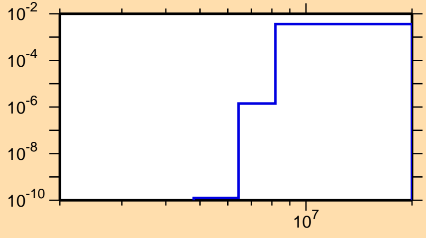
\sigma vs. E for ^{83}\text{Se}(n,p)
