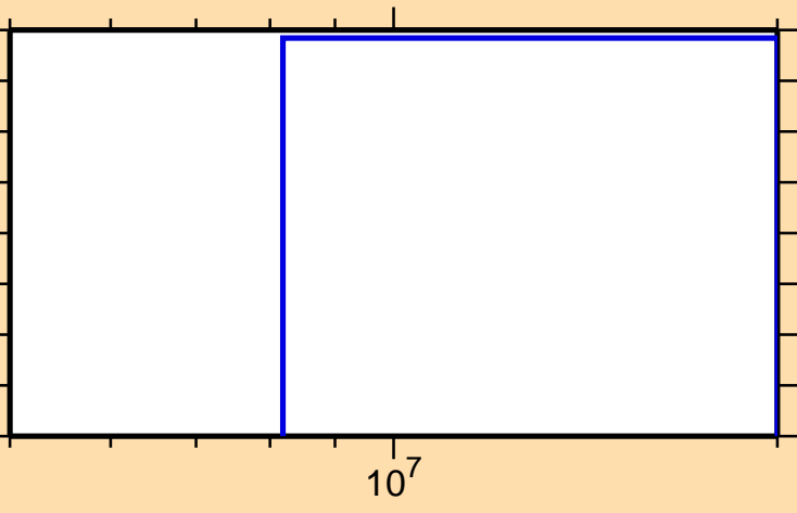
\sigma vs. E for ^{83}\text{Se}(n,\text{nd})
