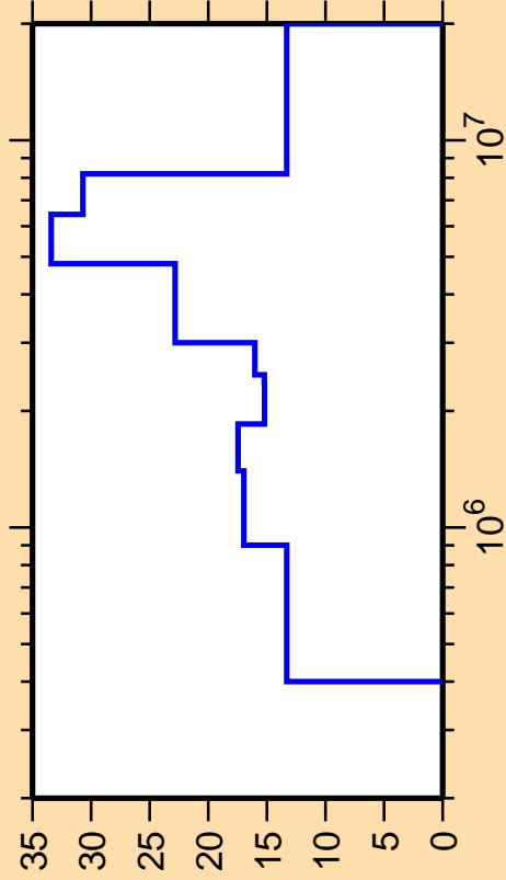
\Delta\sigma/\sigma vs. E for ^{83}\text{Se}(n,n_4)
