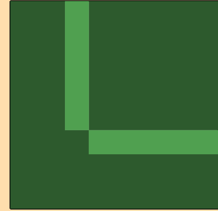
Correlation Matrix
