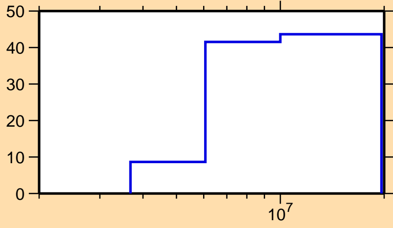
\Delta\sigma/\sigma vs. E for ^{83}\text{Se}(n,p)
