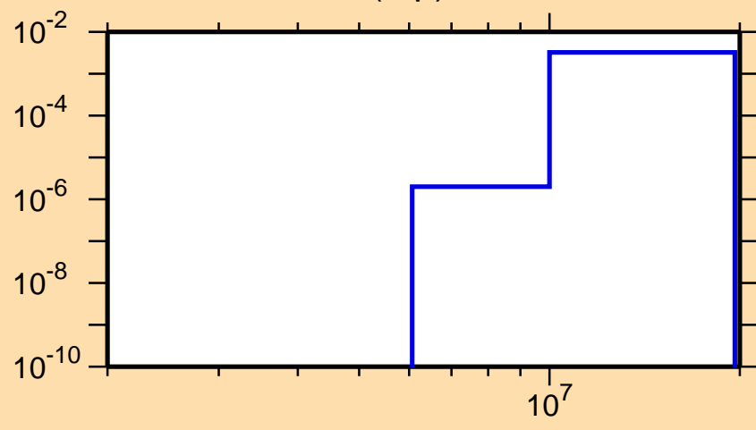
\sigma vs. E for ^{83}\text{Se}(n,p)
