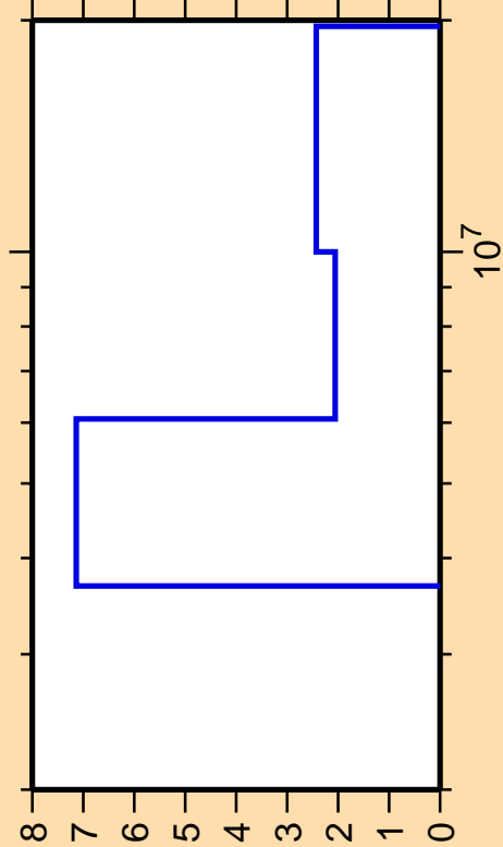
\Delta\sigma/\sigma vs. E for ^{83}\text{Se}(n,2n)
