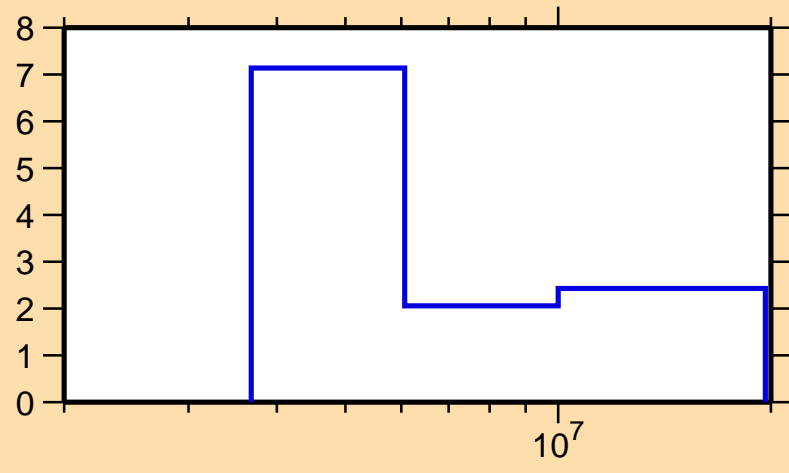
\Delta\sigma/\sigma vs. E for ^{83}\text{Se}(n,2n)
