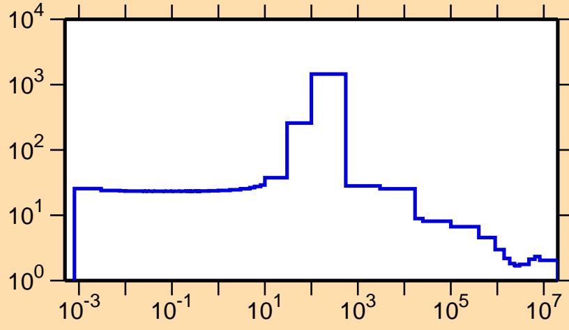
\sigma vs. E for ^{83}\text{Se}(n,\text{el.})
