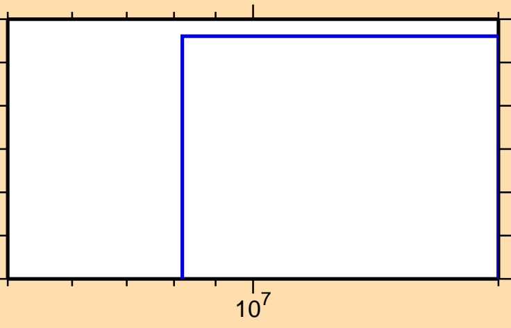
\sigma vs. E for ^{83}\text{Se}(n,\text{nd})
