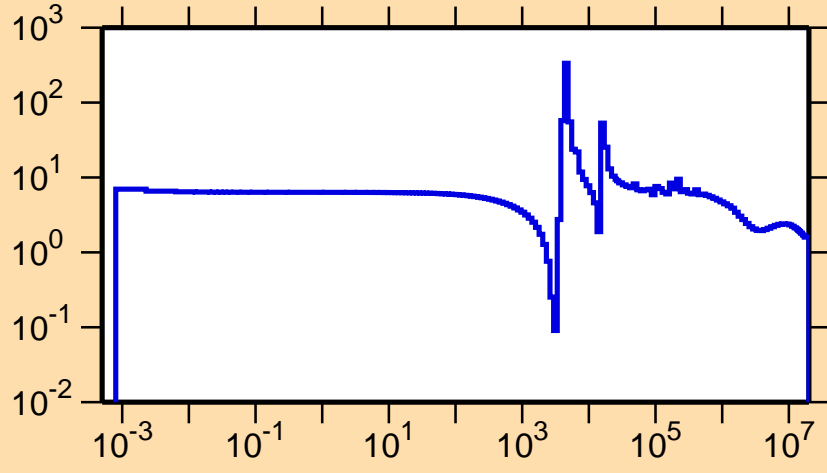
\sigma vs. E for ^{84}\text{Se}(n,\text{el.})
