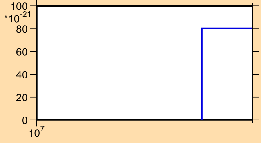
\sigma vs. E for ^{84}\text{Se}(n,nd)
