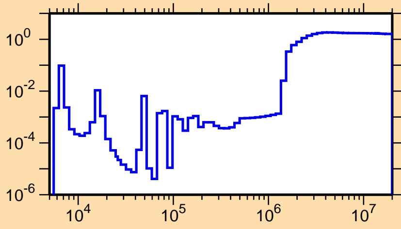
\sigma vs. E for ^{84}\text{Se}(n,\text{nonel.})
