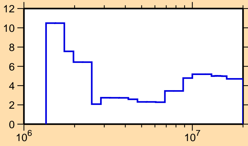
\Delta\sigma/\sigma vs. E for ^{84}\text{Se}(n,\text{tot.})
