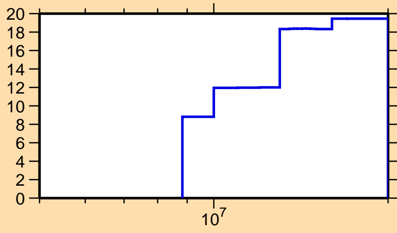
\Delta\sigma/\sigma vs. E for ^{84}\text{Se}(n,\text{inel.})
