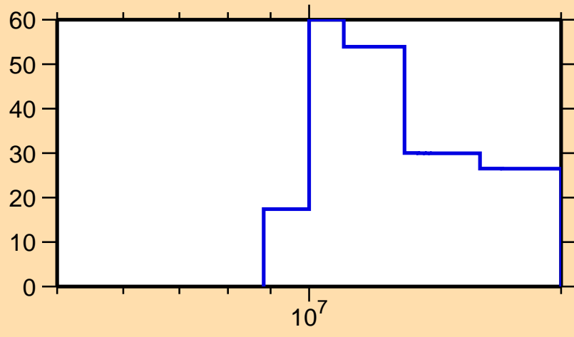
\Delta\sigma/\sigma vs. E for ^{84}\text{Se}(n,p)
