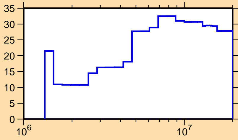
\Delta\sigma/\sigma vs. E for ^{84}\text{Se}(n,n_1)
