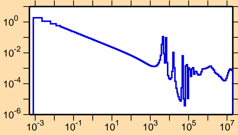
\sigma vs. E for ^{84}\text{Se}(n,\gamma)
