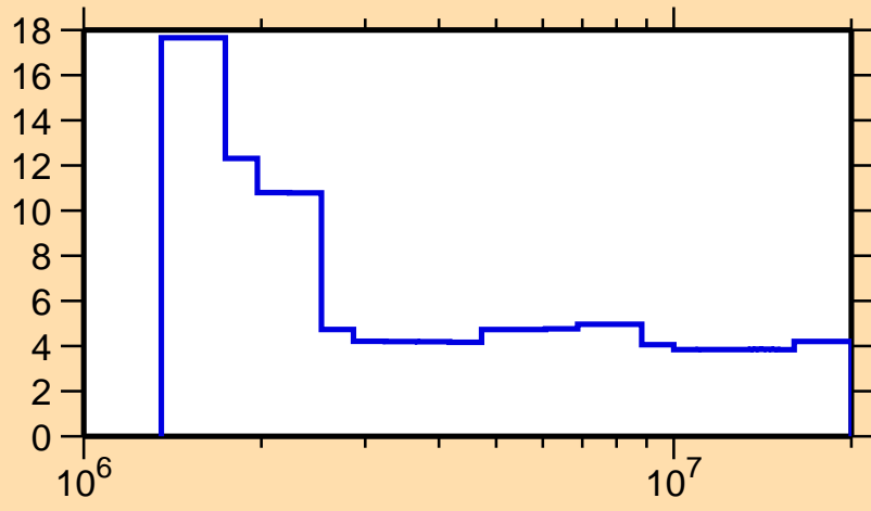
\Delta\sigma/\sigma vs. E for ^{84}\text{Se}(n,\text{nonel.})
