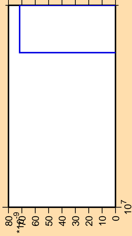
\Delta\sigma/\sigma vs. E for ^{84}\text{Se}(n,nd)
