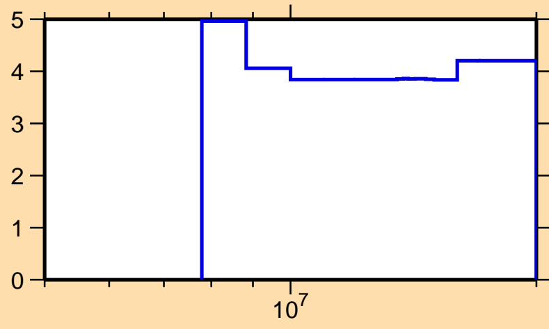
\Delta\sigma/\sigma vs. E for ^{84}\text{Se}(n,\text{nonel.})
