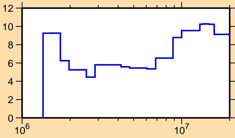
\Delta\sigma/\sigma vs. E for ^{84}\text{Se}(n,\text{el.})
