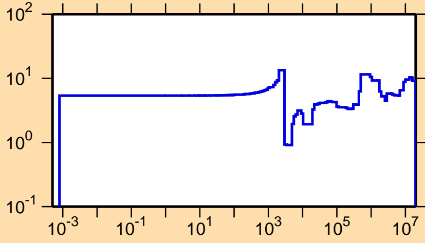
\Delta\sigma/\sigma vs. E for ^{84}\text{Se}(n,\text{el.})
