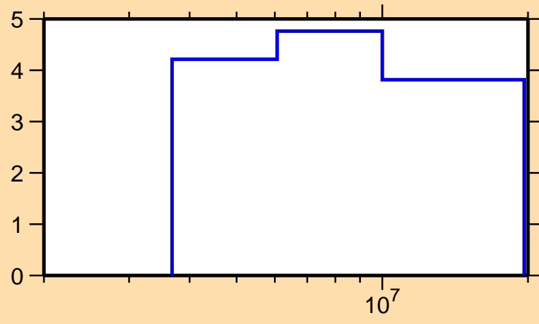
\Delta\sigma/\sigma vs. E for ^{84}\text{Se}(n,n\text{onel.})
