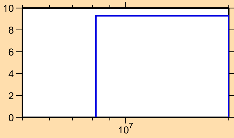
\Delta\sigma/\sigma vs. E for ^{84}\text{Se}(n,el.)
