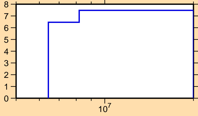
\Delta\sigma/\sigma vs. E for ^{84}\text{Se}(n,n\text{cont.})
