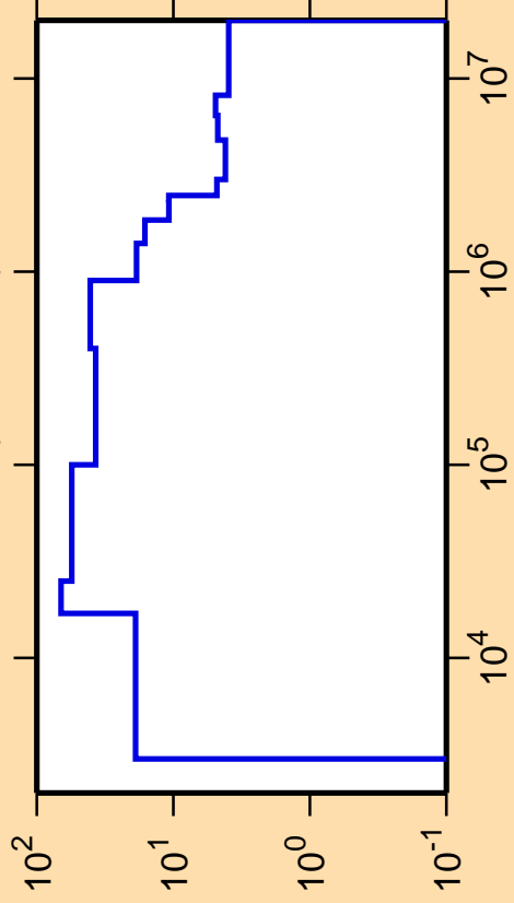
\Delta\sigma/\sigma vs. E for ^{84}\text{Se}(n,\text{nonel.})
