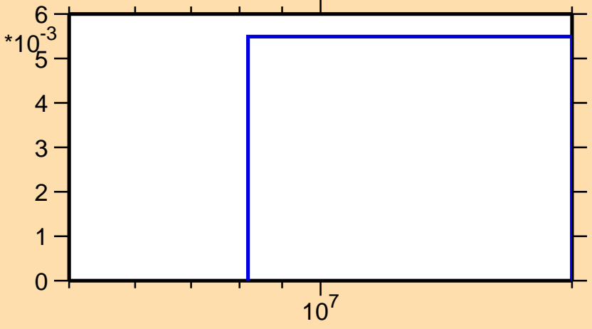
\sigma vs. E for ^{84}\text{Se}(n,3n)
