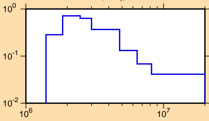
\sigma vs. E for ^{84}\text{Se}(n,n_1)
