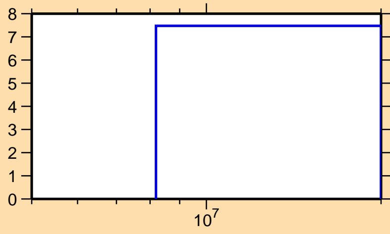
\Delta\sigma/\sigma vs. E for ^{84}\text{Se}(n,ncont.)
