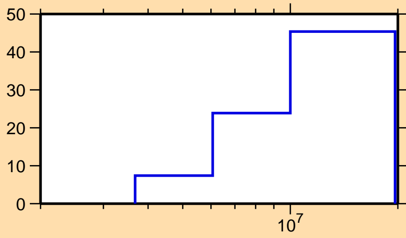
\Delta\sigma/\sigma vs. E for ^{85}\text{Se}(n,\text{inel.})
