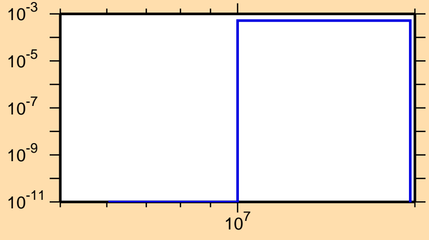
\sigma vs. E for ^{85}\text{Se}(n,p)
