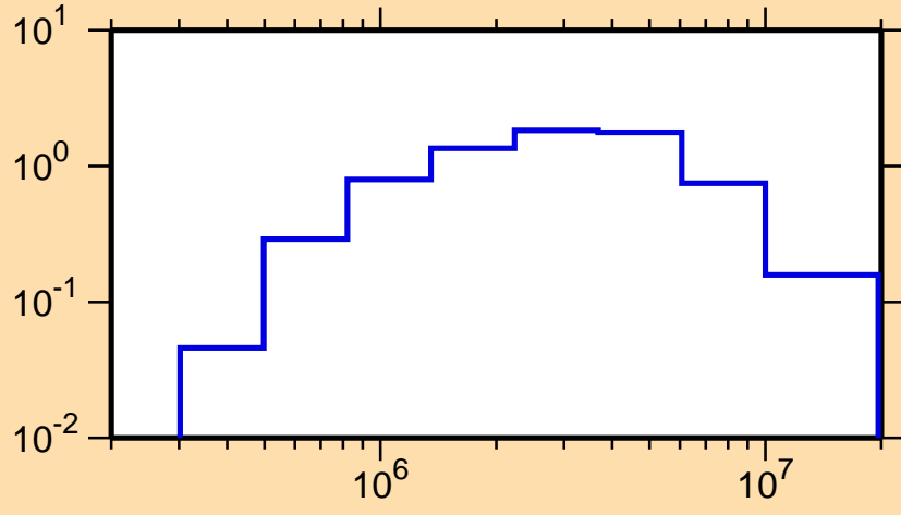
\sigma vs. E for ^{85}\text{Se}(n,n\text{cont.})
