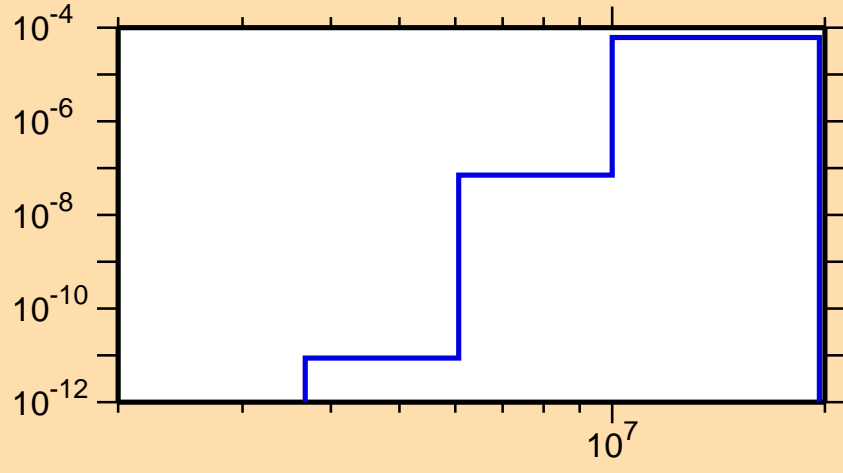
\sigma vs. E for ^{85}\text{Se}(n,\alpha)
