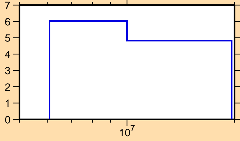
\Delta\sigma/\sigma vs. E for ^{85}\text{Se}(n,\text{nonel.})
