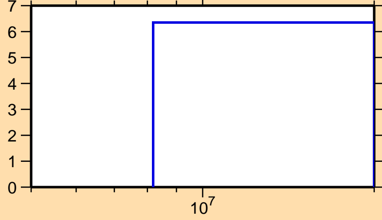
\Delta\sigma/\sigma vs. E for ^{85}\text{Se}(n,\text{tot.})
