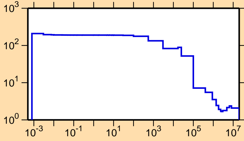
\sigma vs. E for ^{85}\text{Se}(n,\text{el.})
