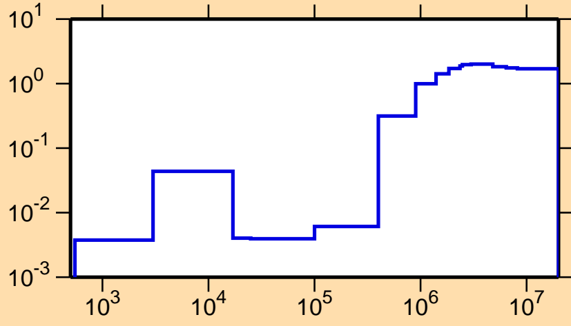
\sigma vs. E for ^{85}\text{Se}(n,\text{nonel.})
