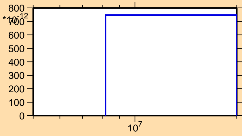
\sigma vs. E for ^{85}\text{Se}(n,\text{nd})
