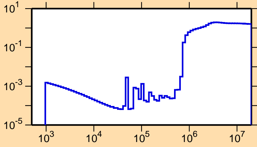
\sigma vs. E for ^{86}\text{Se}(n,\text{nonel.})
