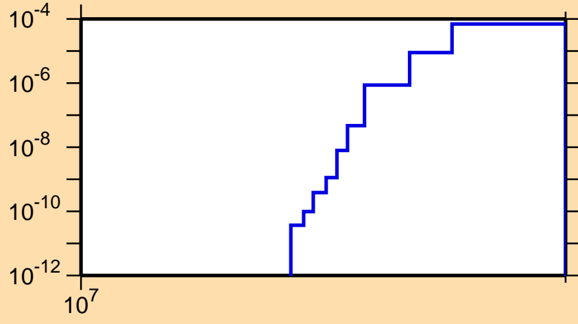
\sigma vs. E for ^{86}\text{Se}(n,t)
