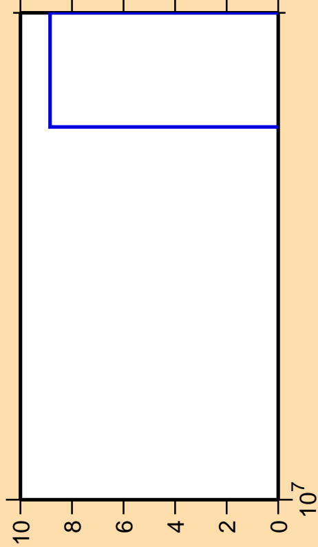
\Delta\sigma/\sigma vs. E for ^{86}\text{Se}(n,nd)
