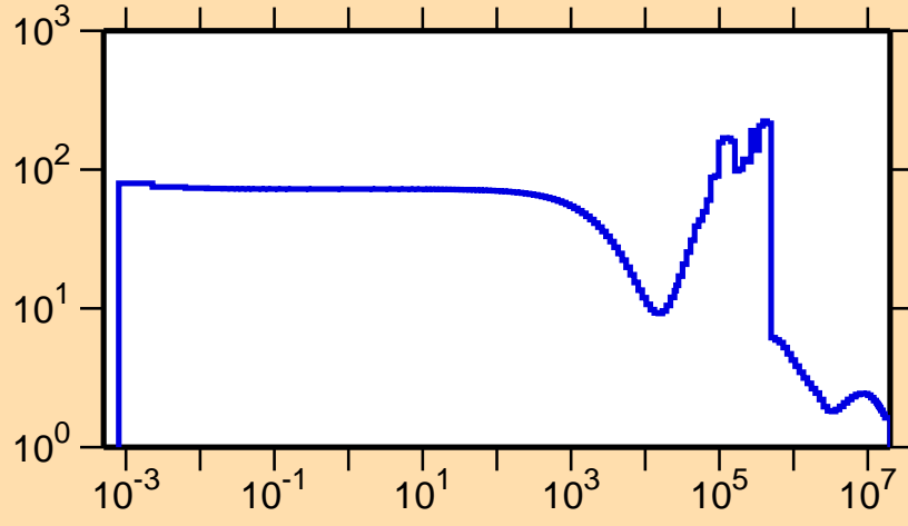
\sigma vs. E for ^{86}\text{Se}(n,\text{el.})
