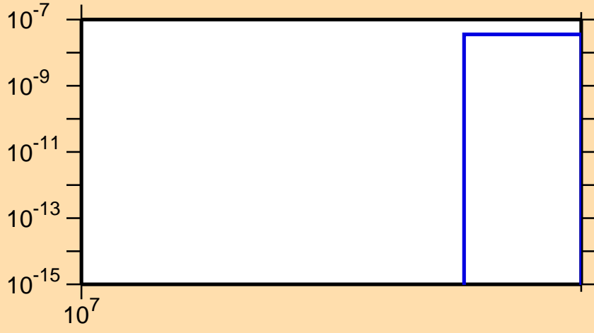
\sigma vs. E for ^{86}\text{Se}(n,nt)
