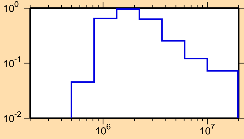
\sigma vs. E for ^{86}\text{Se}(n,n_1)
