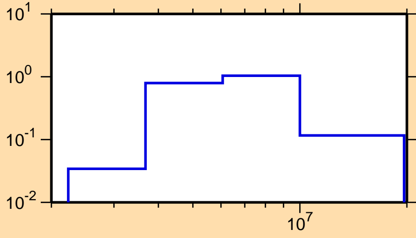
\sigma vs. E for ^{86}\text{Se}(n,n\text{cont.})
