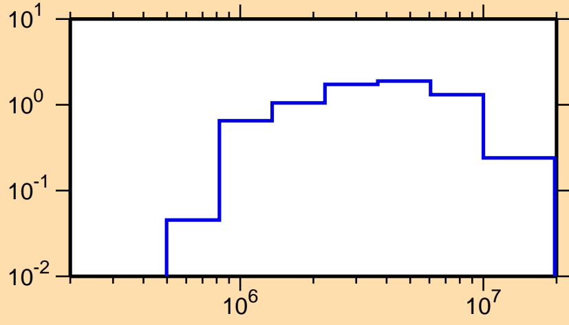
\sigma vs. E for ^{86}\text{Se}(n,\text{inel.})
