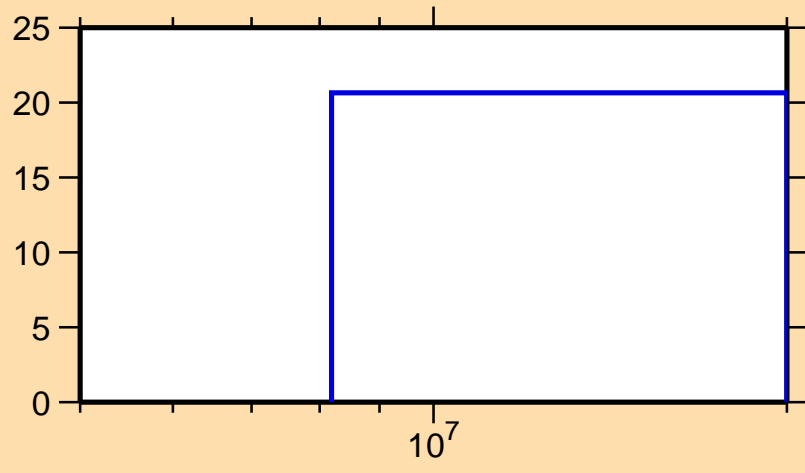
\Delta\sigma/\sigma vs. E for ^{86}\text{Se}(n,ncont.)
