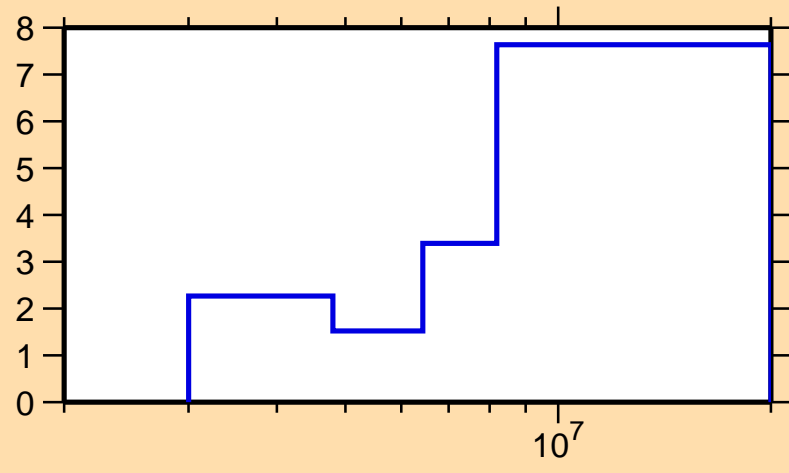
\Delta\sigma/\sigma vs. E for ^{86}\text{Se}(n,\text{tot.})
