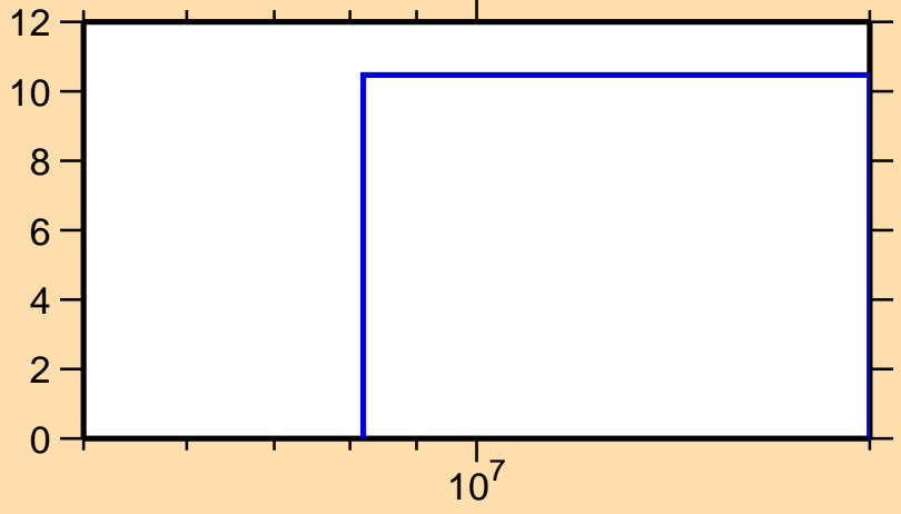
\Delta\sigma/\sigma vs. E for ^{86}\text{Se}(n,el.)
