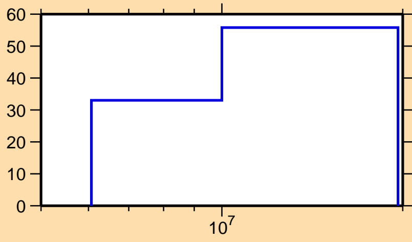
\Delta\sigma/\sigma vs. E for ^{87}\text{Se}(n,ncont.)
