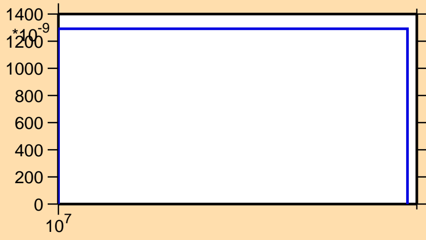
\sigma vs. E for ^{87}\text{Se}(n,d)
