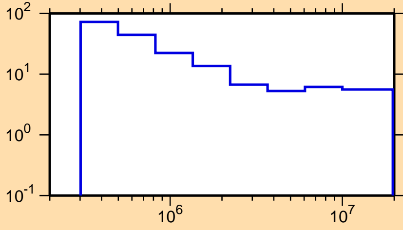
\Delta\sigma/\sigma vs. E for ^{87}\text{Se}(n,n\text{onel.})
