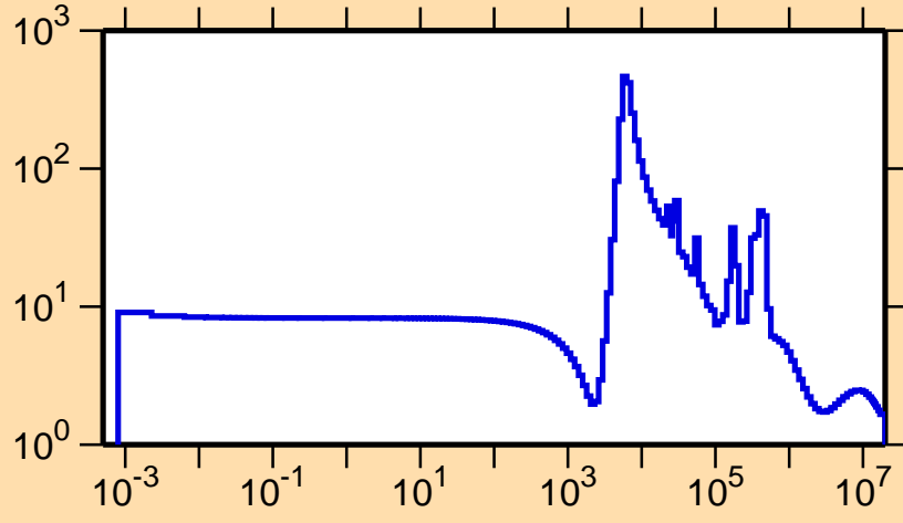
\sigma vs. E for ^{88}\text{Se}(n,\text{el.})
