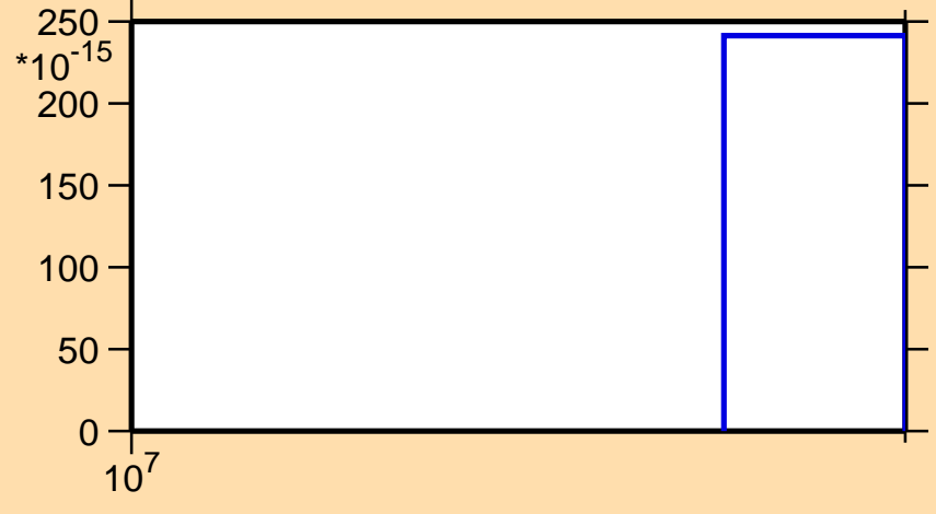
\sigma vs. E for ^{88}\text{Se}(n,nd)
