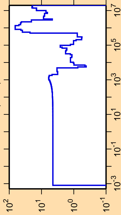
\Delta\sigma/\sigma vs. E for ^{88}\text{Se}(n,\text{el.})
