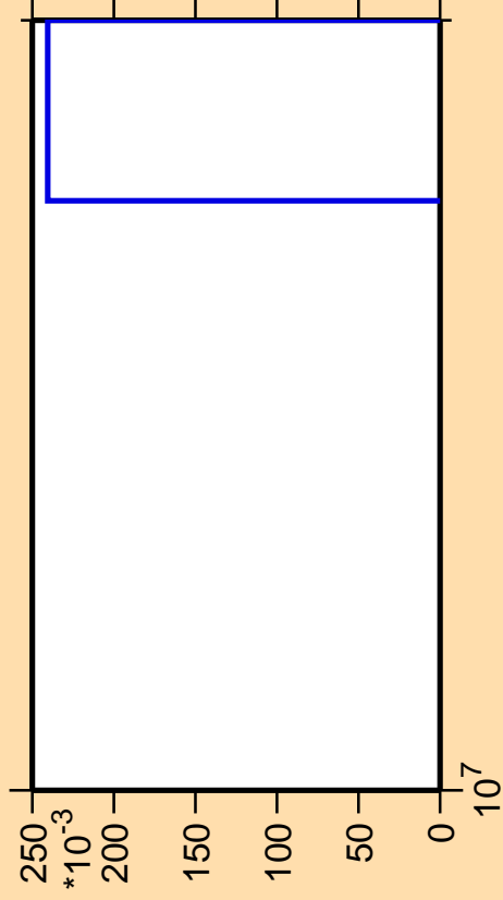
\Delta\sigma/\sigma vs. E for ^{88}\text{Se}(n,nd)
