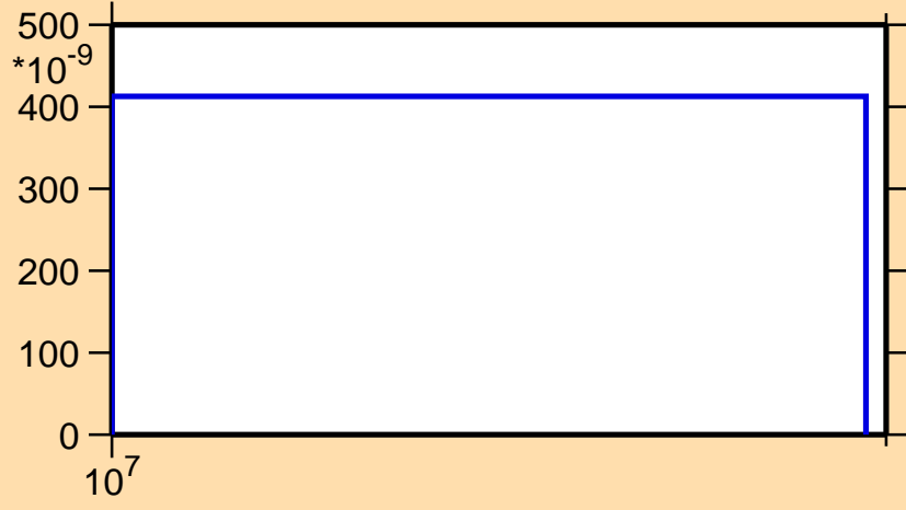
\sigma vs. E for ^{88}\text{Se}(n,p)
