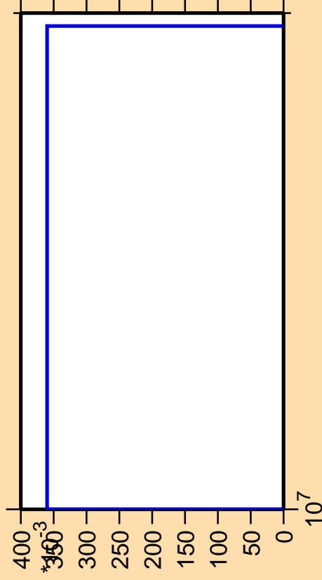
\Delta\sigma/\sigma vs. E for ^{88}\text{Se}(n,2n\alpha)
