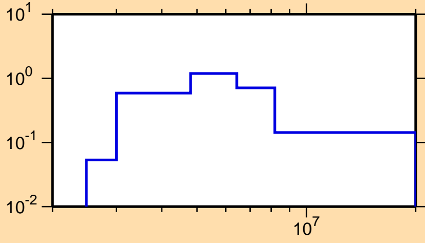
\sigma vs. E for ^{88}\text{Se}(n,n\text{cont.})
