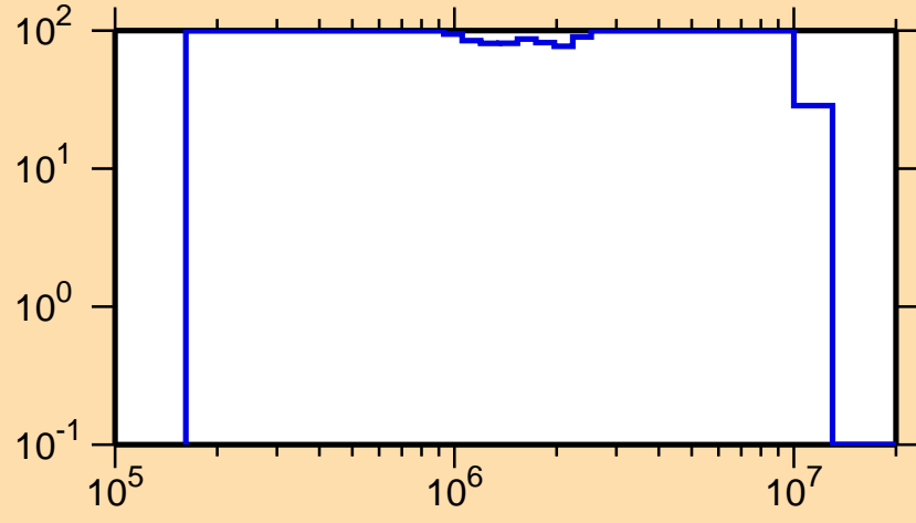
\Delta\sigma/\sigma vs. E for ^{265}\text{Pu}
