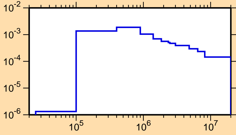
\sigma vs. E for ^{267}\text{Po}
