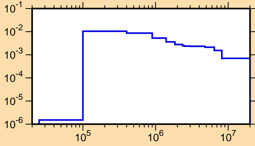
\sigma vs. E for ^{269}_{1} )
