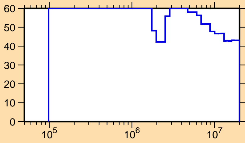
\Delta\sigma/\sigma vs. E for ^{270}_{1}
