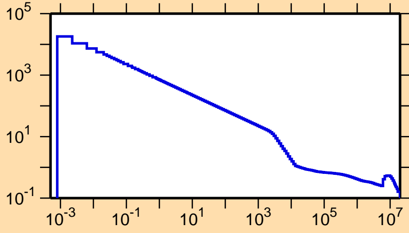
\sigma vs. E for ^{27}\text{Si}(n,\alpha)
