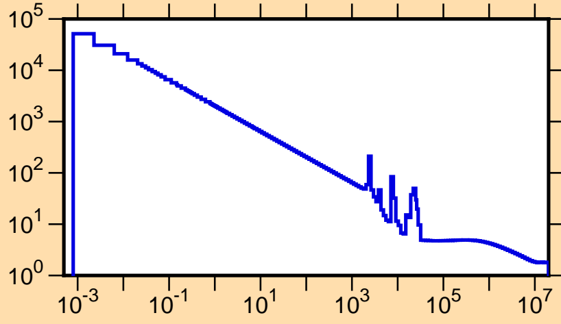
\sigma vs. E for ^{27}\text{Si}(n,\text{tot.})
