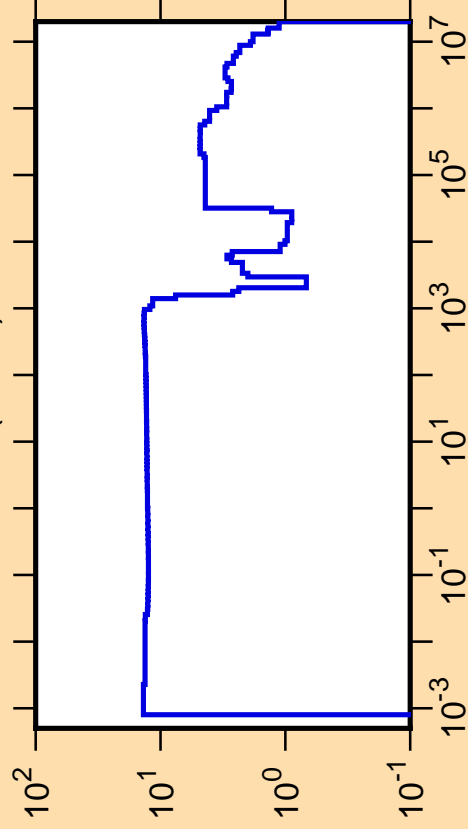
\Delta\sigma/\sigma vs. E for ^{27}\text{Si}(n,\text{tot.})
