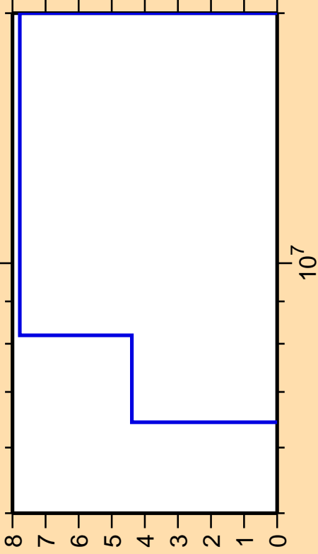
\Delta\sigma/\sigma vs. E for ^{28}\text{Si}(n,n_4)
