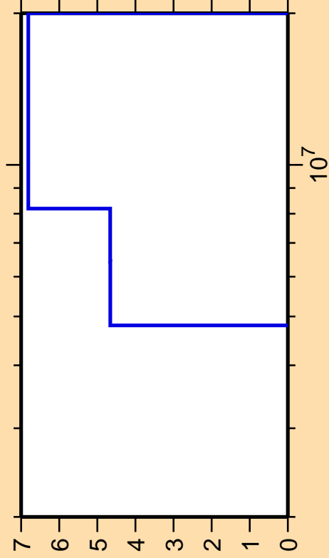
\Delta\sigma/\sigma vs. E for ^{28}\text{Si}(n,n_3)
