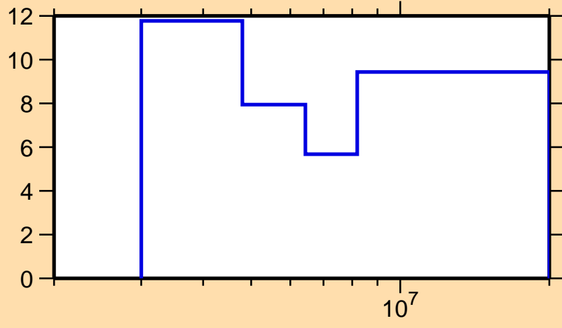
\Delta\sigma/\sigma vs. E for ^{28}\text{Si}(n,p)
