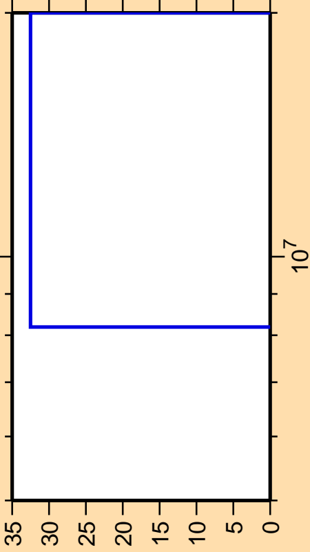
\Delta\sigma/\sigma vs. E for ^{28}\text{Si}(n,\gamma)
