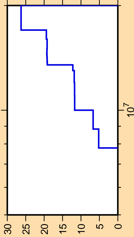
\Delta\sigma/\sigma vs. E for ^{29}\text{Si}(n,n_1)
