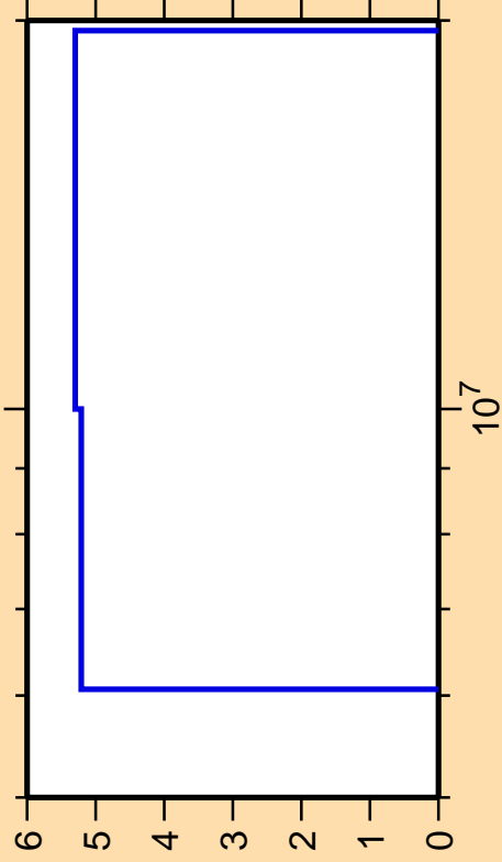
\Delta\sigma/\sigma vs. E for ^{29}\text{Si}(n,p)
