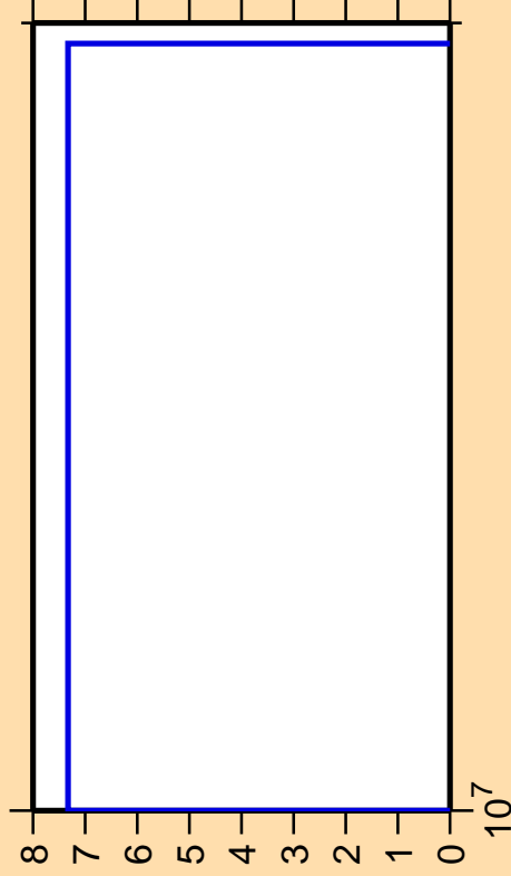
\Delta\sigma/\sigma vs. E for ^{29}\text{Si}(n,np)
