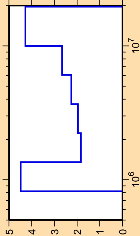
\Delta\sigma/\sigma vs. E for ^{29}\text{Si}(n,\text{inel.})
