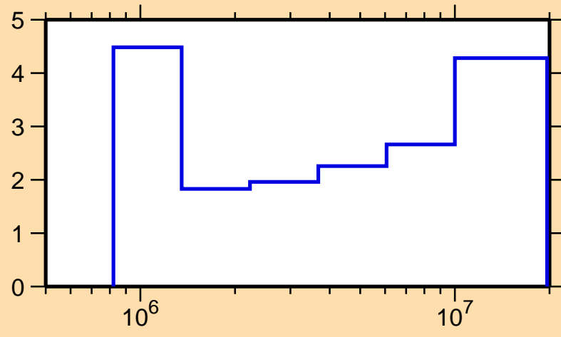
\Delta\sigma/\sigma vs. E for ^{29}\text{Si}(n,\text{inel.})
