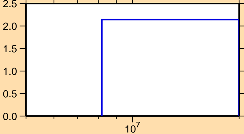
\Delta\sigma/\sigma vs. E for ^{30}\text{Si}(n,\text{tot.})
