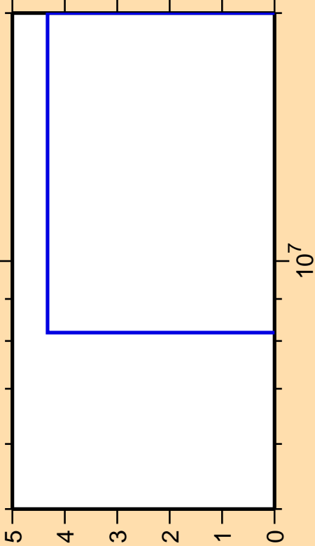
\Delta\sigma/\sigma vs. E for ^{30}\text{Si}(n,2n)
