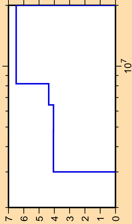
\Delta\sigma/\sigma vs. E for ^{30}\text{Si}(n,n_4)
