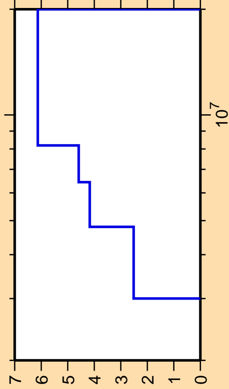
\Delta\sigma/\sigma vs. E for ^{30}\text{Si}(n,n_2)
