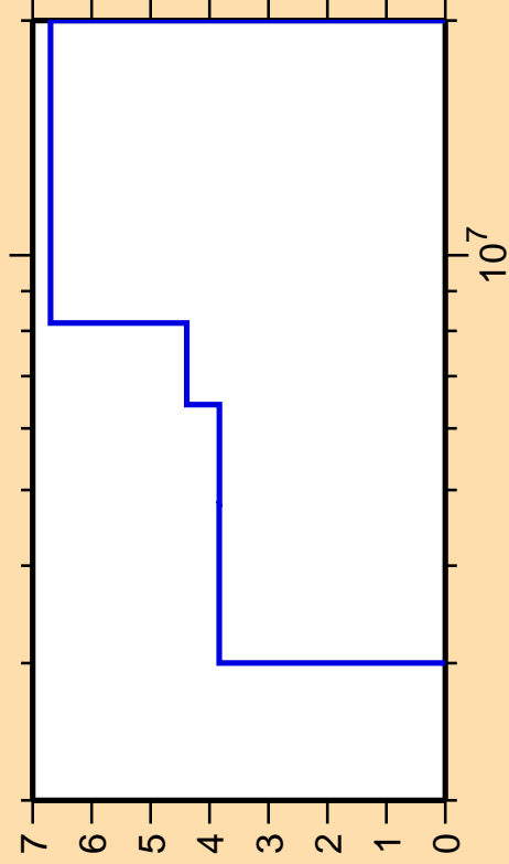
\Delta\sigma/\sigma vs. E for ^{30}\text{Si}(n,n_3)
