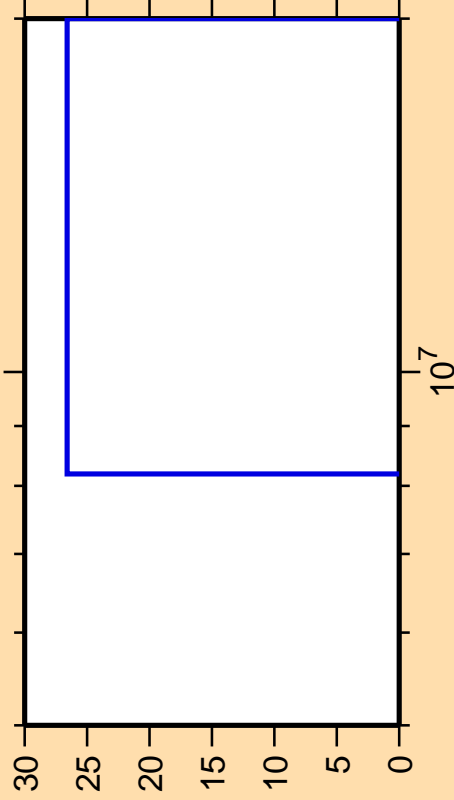
\Delta\sigma/\sigma vs. E for ^{30}\text{Si}(n,\gamma)
