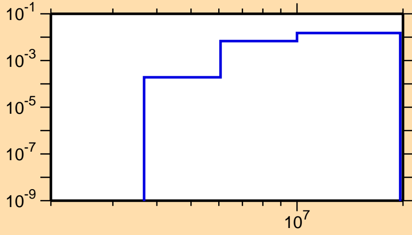
\sigma vs. E for ^{31}\text{Si}(n,\alpha)
