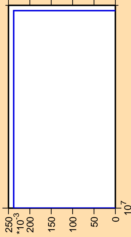
\Delta\sigma/\sigma vs. E for ^{31}\text{Si}(n,2n\alpha)
