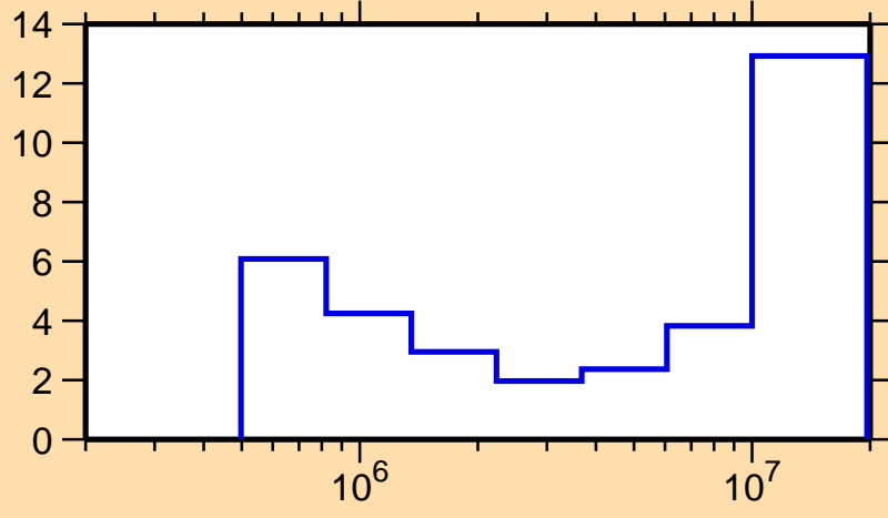
\Delta\sigma/\sigma vs. E for ^{31}\text{Si}(n,n_1)
