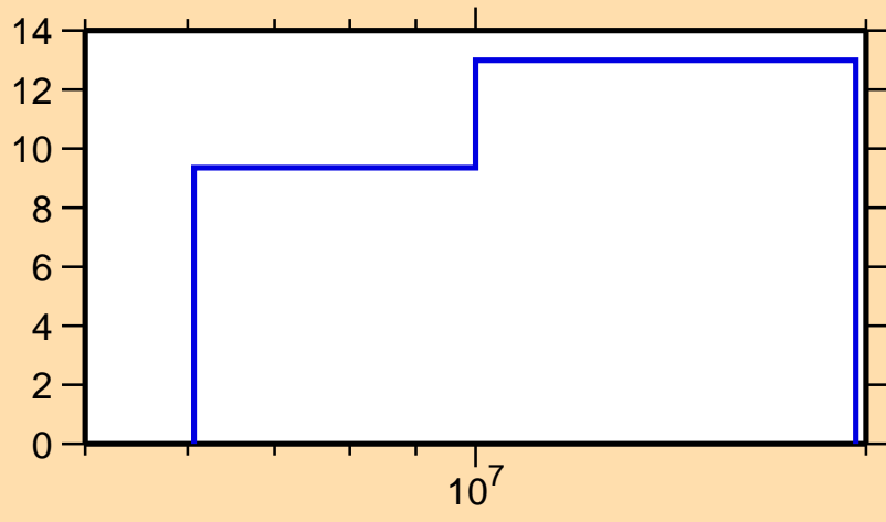
\Delta\sigma/\sigma vs. E for ^{31}\text{Si}(n,ncont.)
