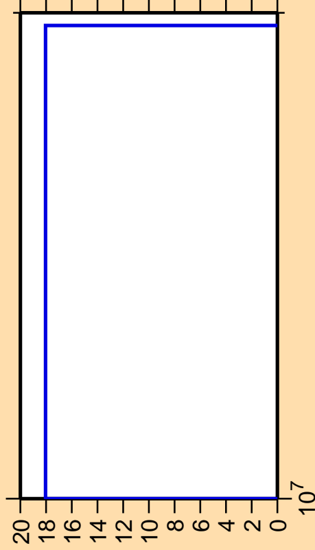
\Delta\sigma/\sigma vs. E for ^{31}\text{Si}(n,t)
