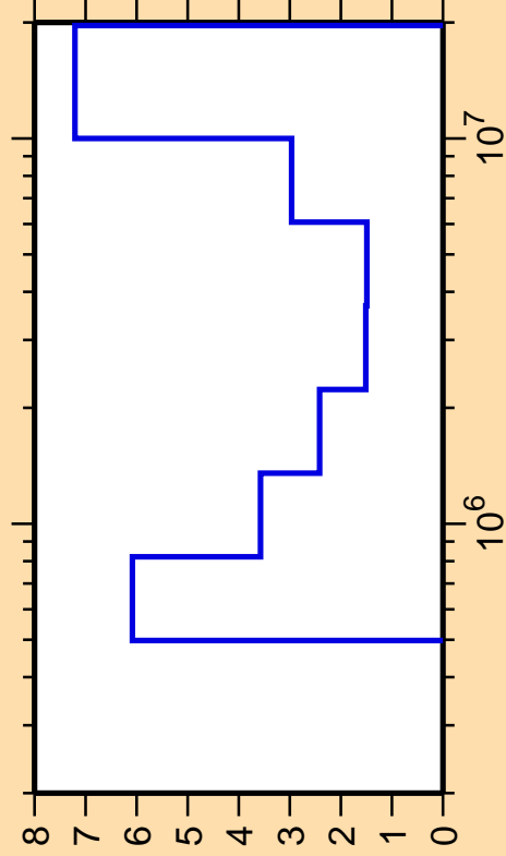
\Delta\sigma/\sigma vs. E for ^{31}\text{Si}(n,\text{inel.})
