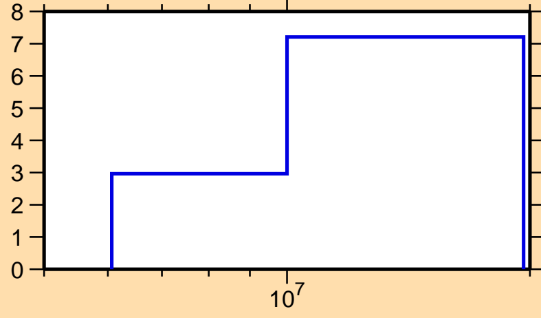
\Delta\sigma/\sigma vs. E for ^{31}\text{Si}(n,\text{inel.})
