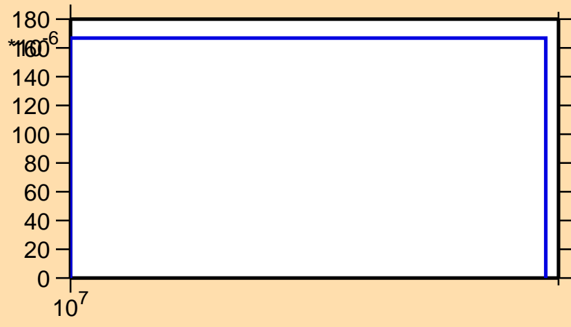
\sigma vs. E for ^{31}\text{Si}(n,t)
