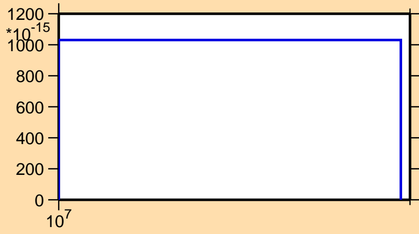
\sigma vs. E for ^{31}\text{Si}(n,2n\alpha)
