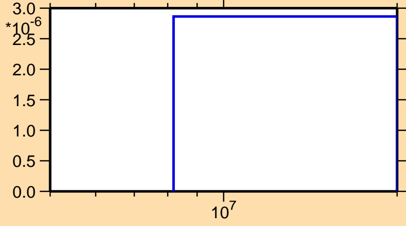
\sigma vs. E for ^{31}\text{Si}(n,3n)
