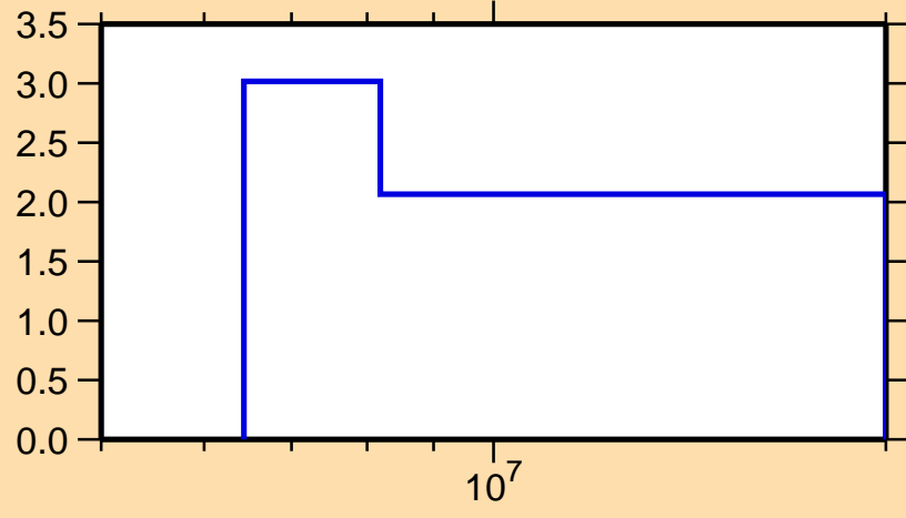
\Delta\sigma/\sigma vs. E for ^{31}\text{Si}(n,el.)
