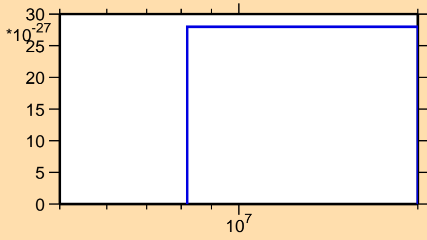
\sigma vs. E for ^{31}\text{Si}(n,p\alpha)
