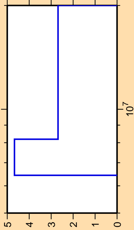
\Delta\sigma/\sigma vs. E for ^{31}\text{Si}(n,2n)
