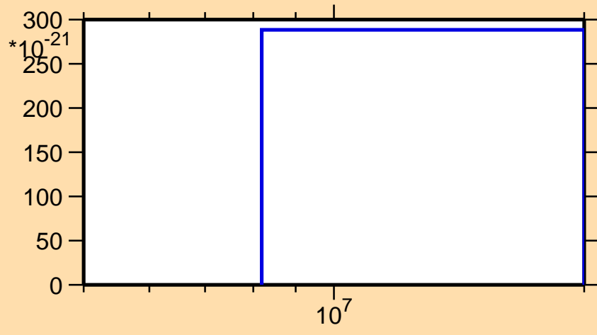
\sigma vs. E for ^{31}\text{Si}(n,\text{He}3)
