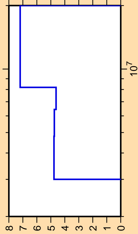
\Delta\sigma/\sigma vs. E for ^{32}\text{Si}(n,n_2)
