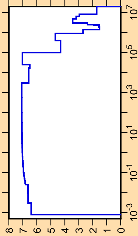
\Delta\sigma/\sigma vs. E for ^{32}\text{Si}(n,\text{tot.})
