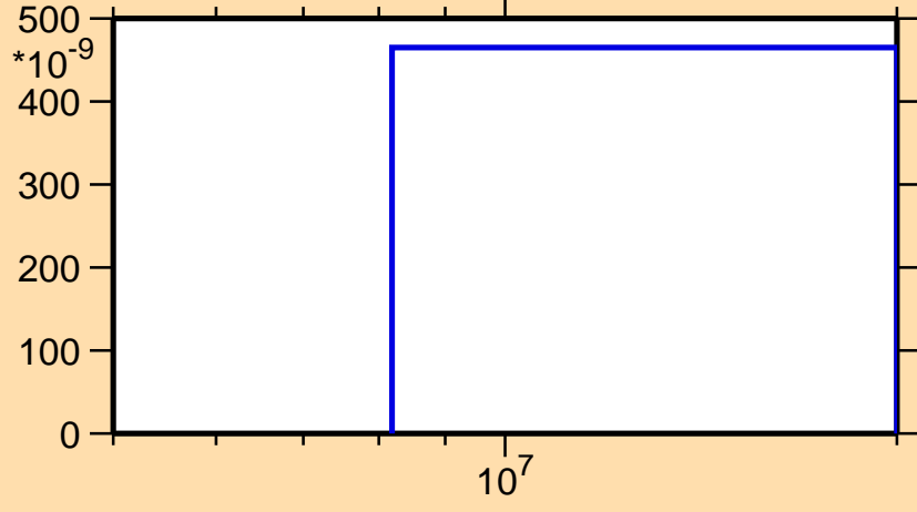
\sigma vs. E for ^{32}\text{Si}(n,t)
