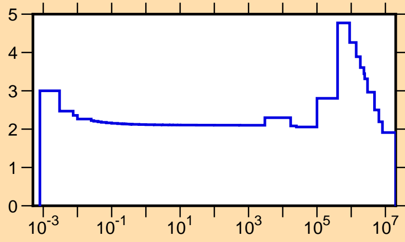
\sigma vs. E for ^{32}\text{Si}(n,\text{tot.})
