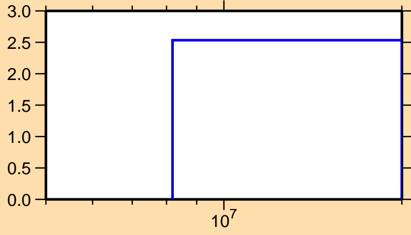
\Delta\sigma/\sigma vs. E for ^{32}\text{Si}(n,n\text{onel.})
