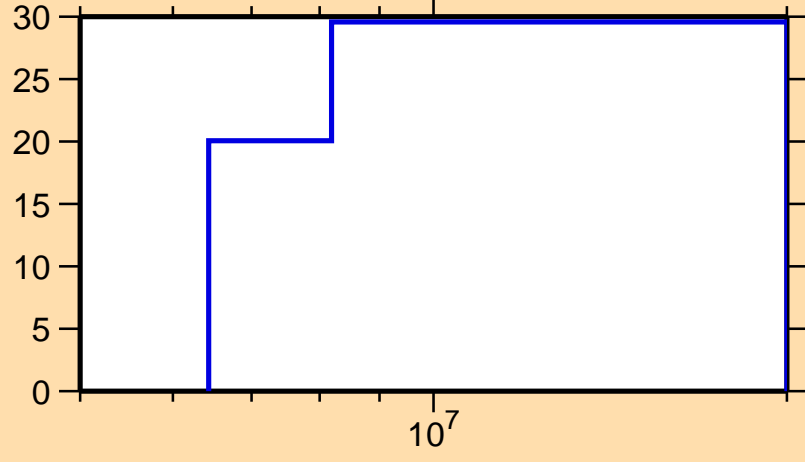
\Delta\sigma/\sigma vs. E for ^{32}\text{Si}(n,\gamma)
