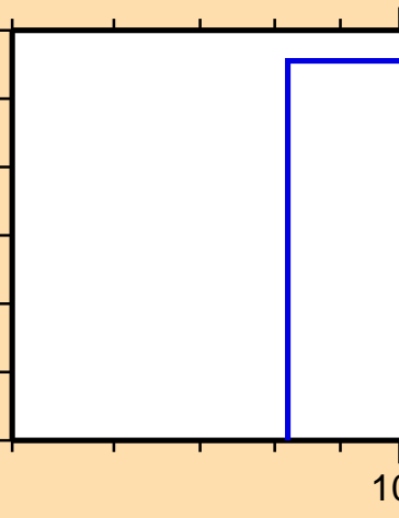
\sigma vs. E for ^{32}\text{Si}(n,d)
