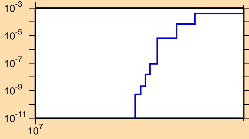
\sigma vs. E for ^{33}\text{Si}(n,n\alpha)
