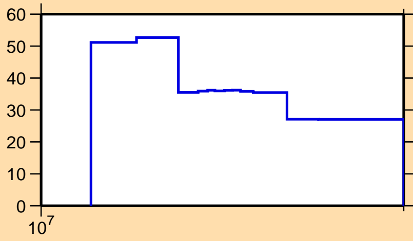
\Delta\sigma/\sigma vs. E for ^{33}\text{Si}(n,ncont.)
