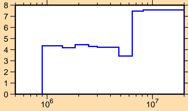
\Delta\sigma/\sigma vs. E for ^{33}\text{Si}(n,\text{inel.})
