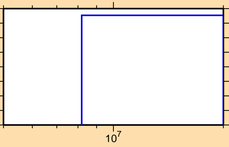
\sigma vs. E for ^{33}\text{Si}(n,np)
