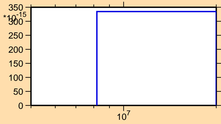
\sigma vs. E for ^{33}\text{Si}(n,nd)
