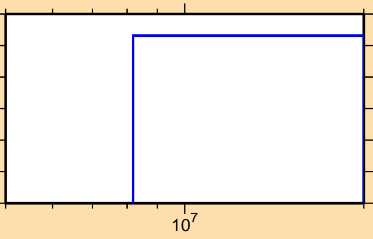
\sigma vs. E for ^{33}\text{Si}(n,d)
