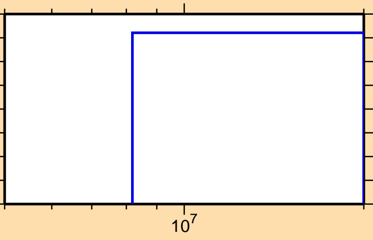
\sigma vs. E for ^{33}\text{Si}(n,3n)
