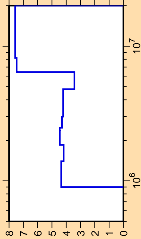
\Delta\sigma/\sigma vs. E for ^{33}\text{Si}(n,\text{inel.})
