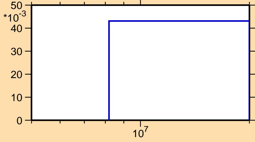
\sigma vs. E for ^{34}\text{Si}(n,3n)
