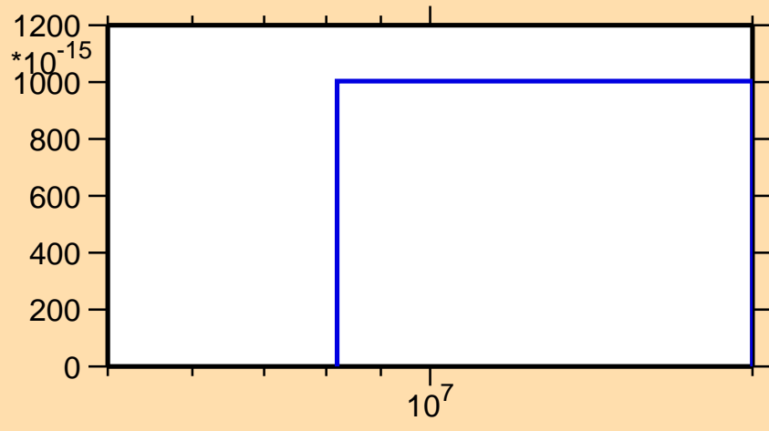
\sigma vs. E for ^{34}\text{Si}(n,np)
