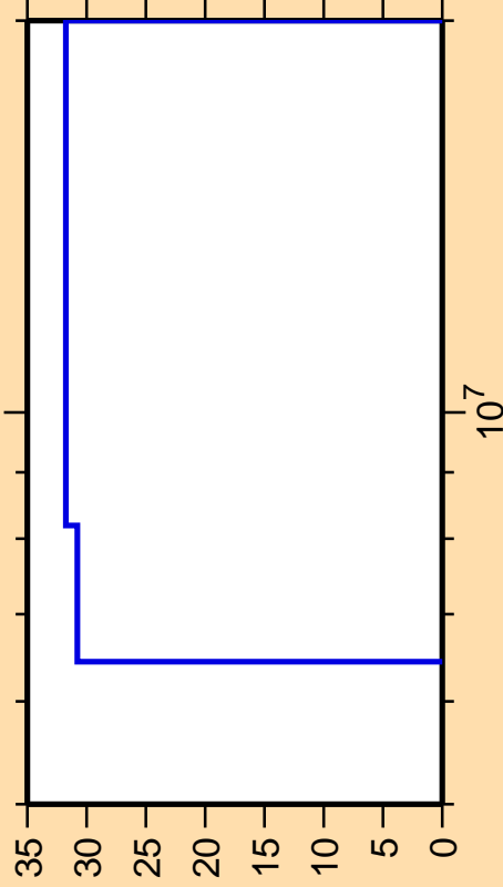
\Delta\sigma/\sigma vs. E for ^{34}\text{Si}(n,\gamma)
