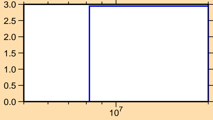
\Delta\sigma/\sigma vs. E for ^{34}\text{Si}(n,el.)
