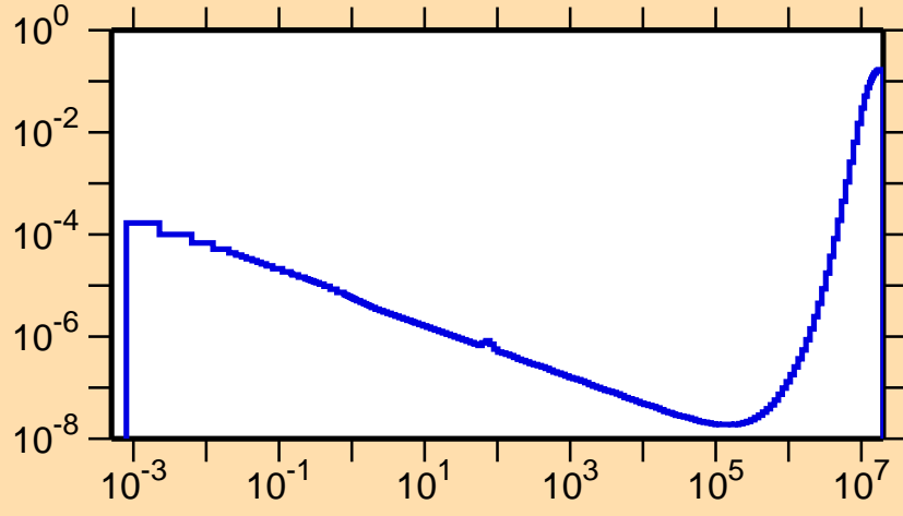
\sigma vs. E for ^{130}\text{Sm}(n,p\alpha)
