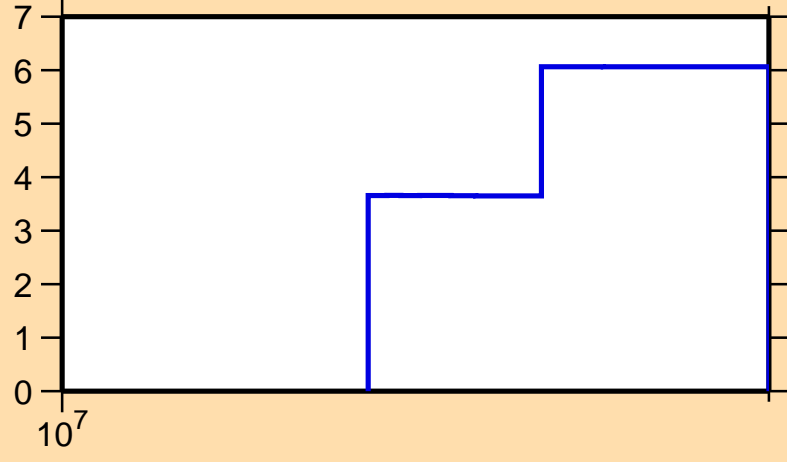
\Delta\sigma/\sigma vs. E for ^{130}\text{Sm}(n,\text{tot.})
