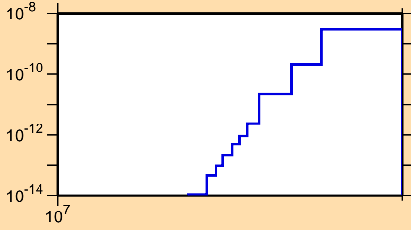
\sigma vs. E for ^{130}\text{Sm} (mt 34)
