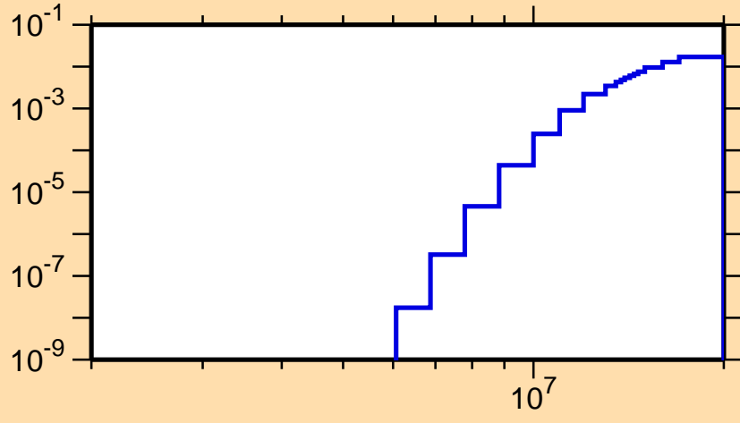
\sigma vs. E for ^{130}\text{Sm}(n,pd)
