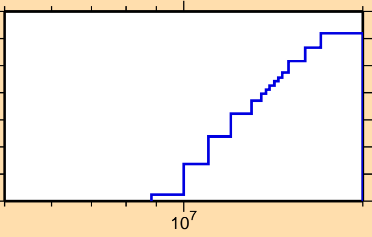
\sigma vs. E for ^{130}\text{Sm}(\text{mt117})
