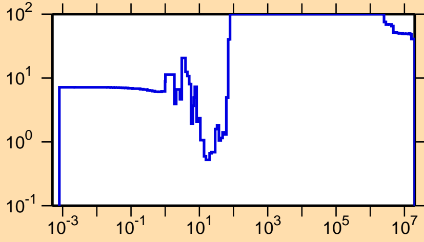
\Delta\sigma/\sigma vs. E for ^{130}\text{Sm}(n,\gamma)
