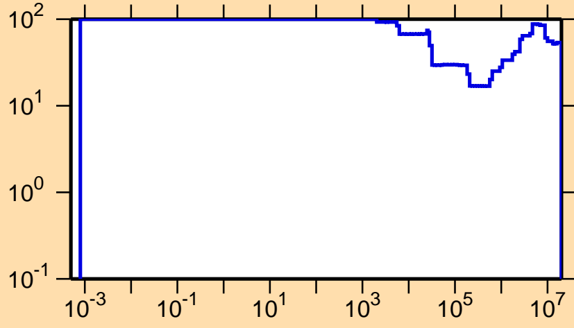
\Delta\sigma/\sigma vs. E for ^{130}\text{Sm}(n,p)
