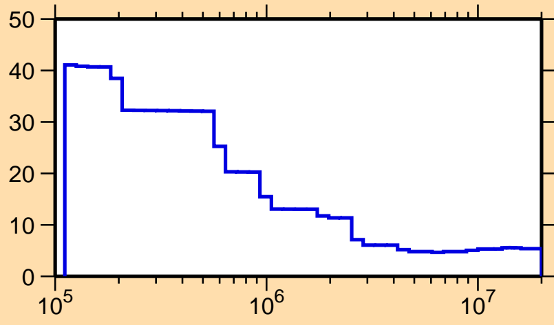
\Delta\sigma/\sigma vs. E for ^{130}\text{Sm}(n,\text{nonel.})
