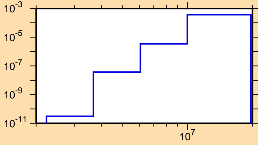
\sigma vs. E for ^{130}\text{Sm}(n,n\alpha)
