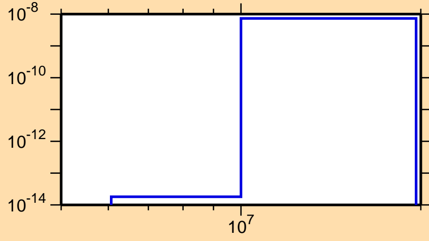
\sigma vs. E for ^{130}\text{Sm}(\text{mt117})
