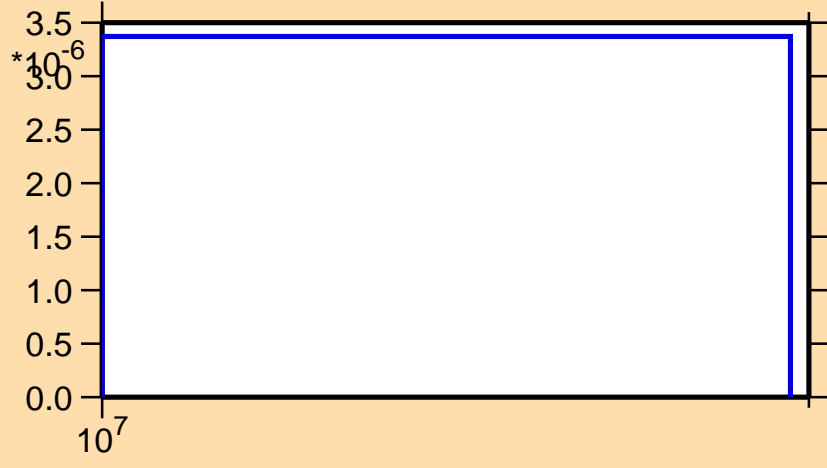
\sigma vs. E for ^{130}\text{Sm}(n,2n)
