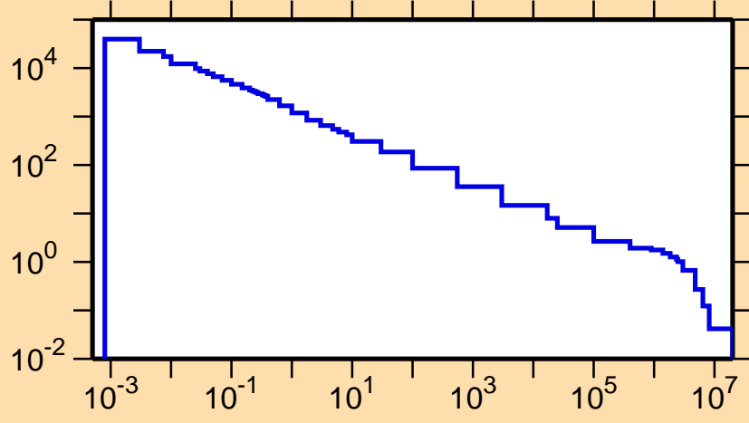
\sigma vs. E for ^{130}\text{Sm}(n,p)
