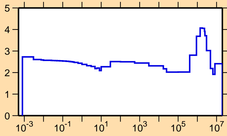
\sigma vs. E for ^{130}\text{Sm}(n,\text{el.})
