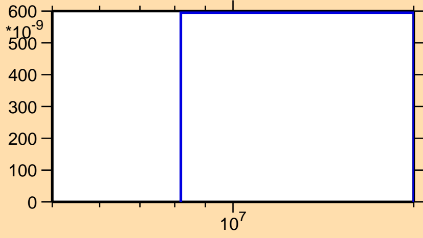
\sigma vs. E for ^{130}\text{Sm} (mt 45)
