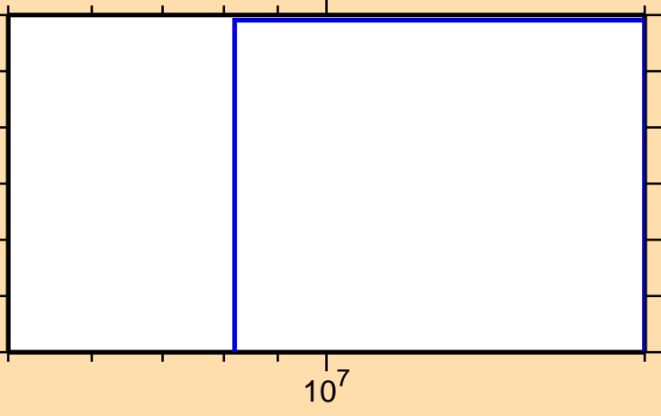
\sigma vs. E for ^{130}\text{Sm}(\text{mt117})
