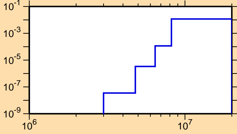
\sigma vs. E for ^{130}\text{Sm}(n,d)
