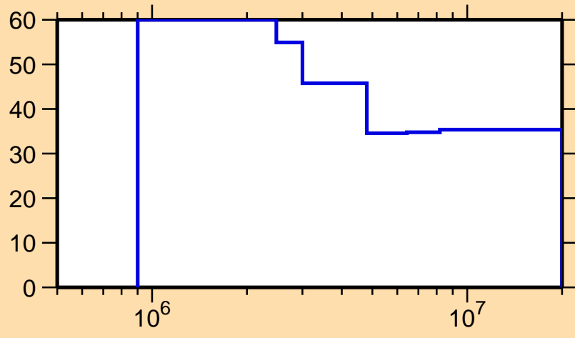
\Delta\sigma/\sigma vs. E for ^{130}\text{Sm}(n,n\text{cont.})
