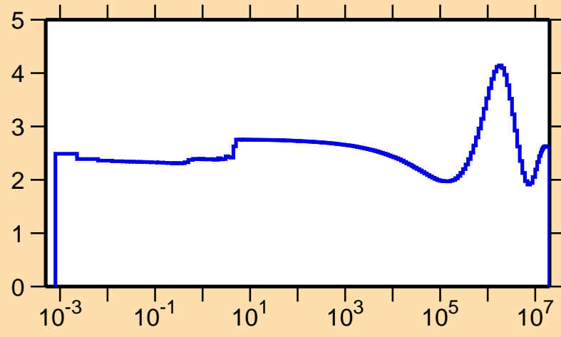
\sigma vs. E for ^{131}\text{Sm}(n,\text{el.})
