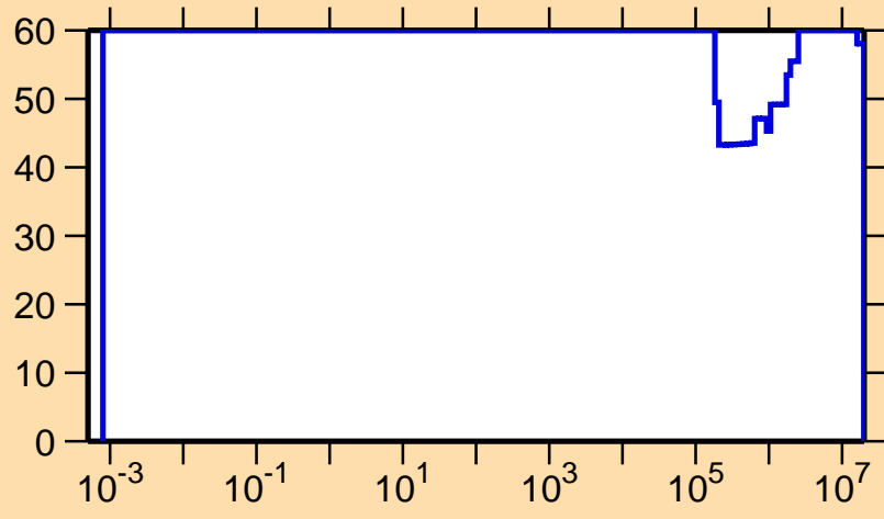
\Delta\sigma/\sigma vs. E for ^{131}\text{Sm}(n,p)
