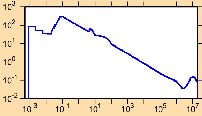
\sigma vs. E for ^{131}\text{Sm}(n,\alpha)
