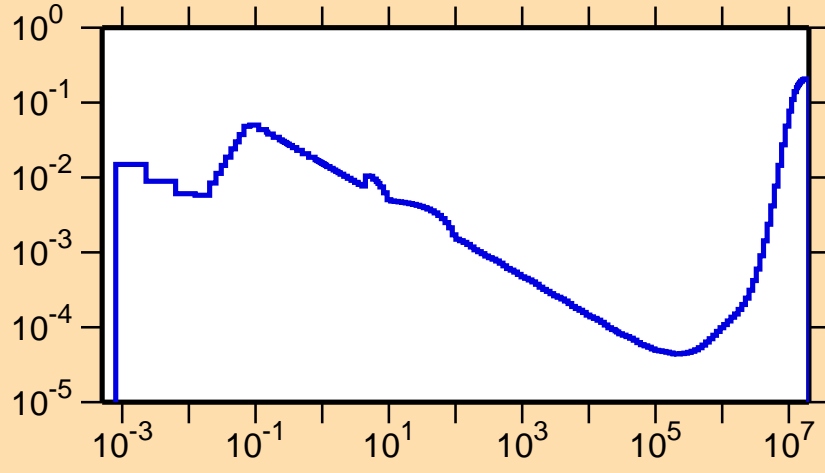
\sigma vs. E for ^{131}\text{Sm}(n,p\alpha)
