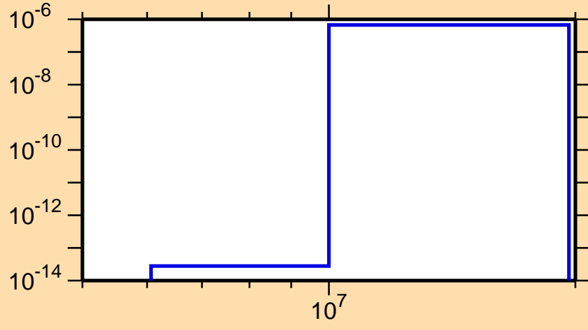
\sigma vs. E for ^{131}\text{Sm} (mt 45)
