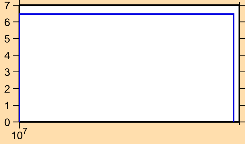
\Delta\sigma/\sigma vs. E for ^{131}\text{Sm}(n,\text{tot.})
