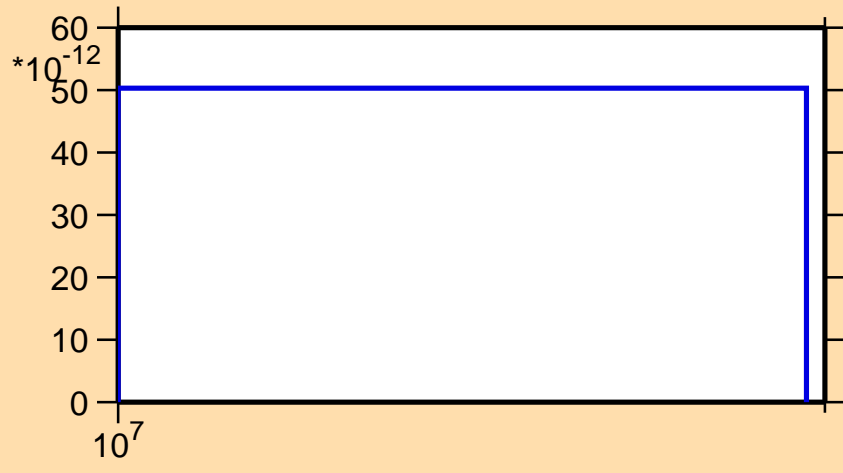
\sigma vs. E for ^{131}\text{Sm}(n,2n\alpha)
