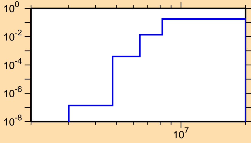
\sigma vs. E for ^{131}\text{Sm}(n,np)
