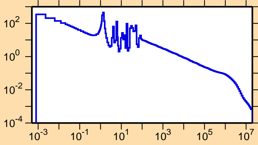
\sigma vs. E for ^{132}\text{Sm}(n,\gamma)
