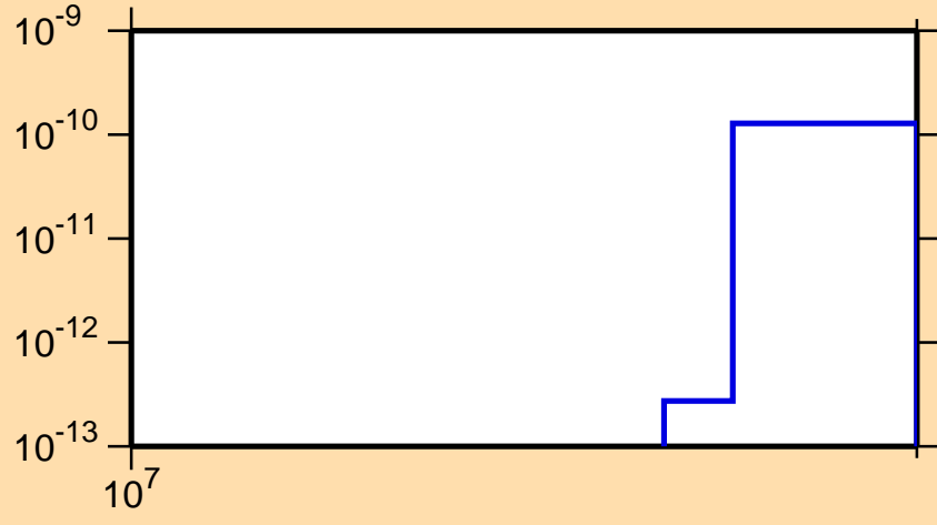
\sigma vs. E for ^{132}\text{Sm}(n,2n\alpha)
