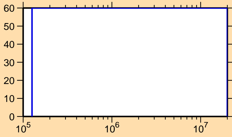
\Delta\sigma/\sigma vs. E for ^{132}\text{Sm}(n,n_1)
