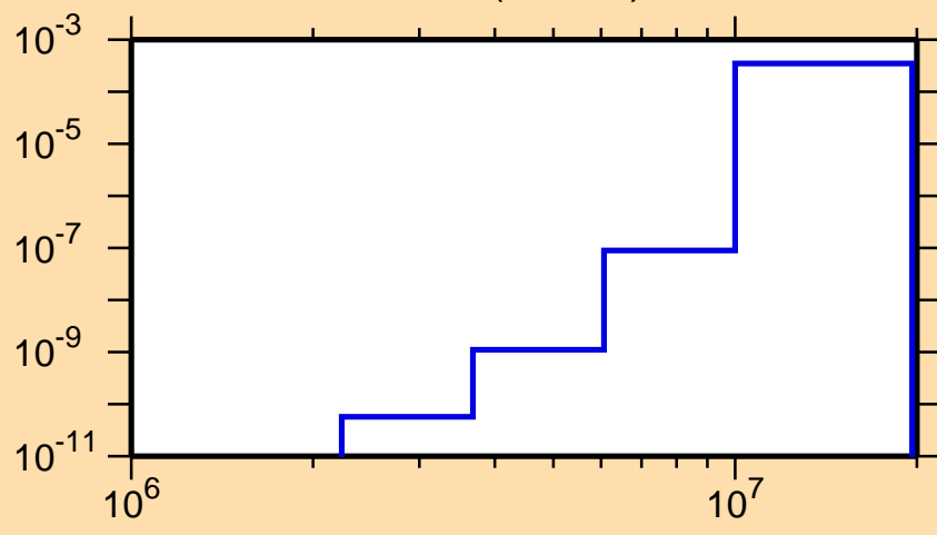
\sigma vs. E for ^{132}\text{Sm}(n,\text{He}3)
