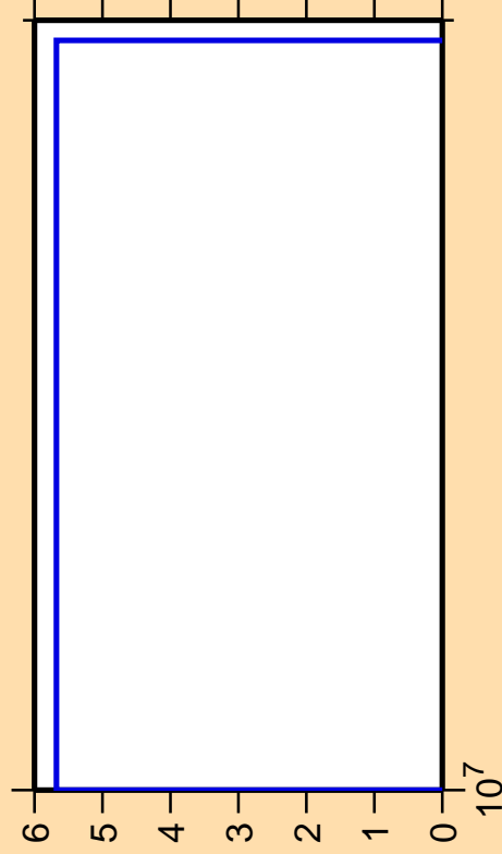
\Delta\sigma/\sigma vs. E for ^{132}\text{Sm}(n,2n\alpha)
