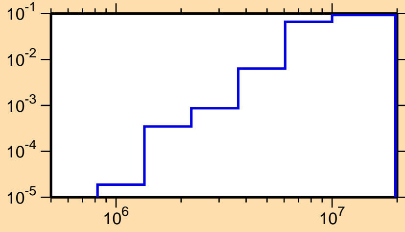
\sigma vs. E for ^{132}\text{Sm}(n,n\text{cont.})
