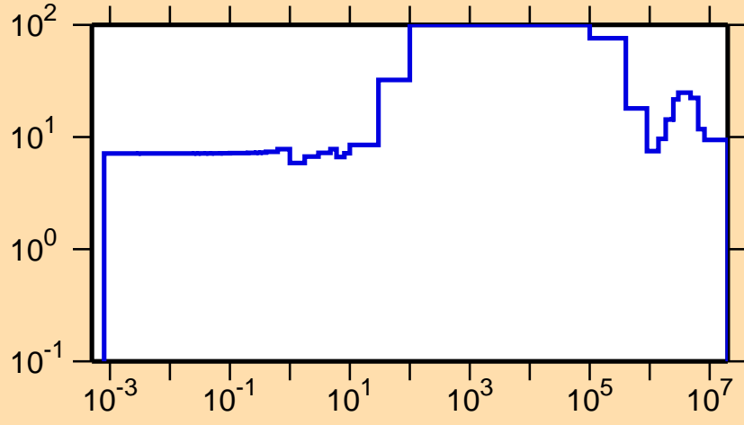
\Delta\sigma/\sigma vs. E for ^{132}\text{Sm}(n,el.)
