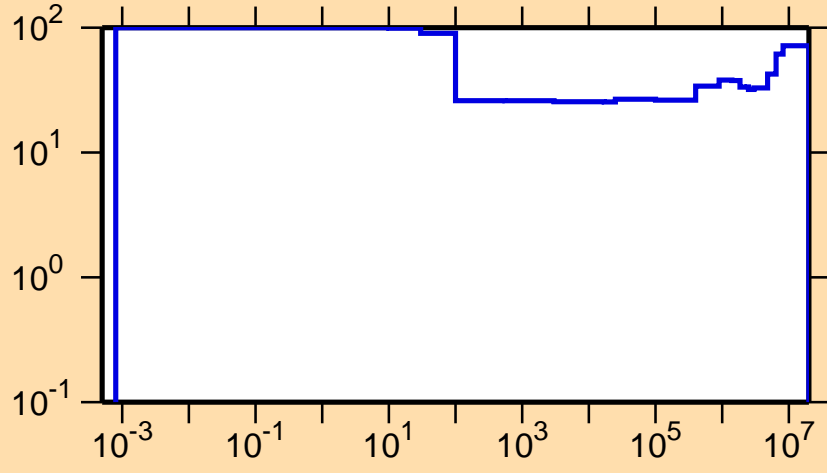
\Delta\sigma/\sigma vs. E for ^{132}\text{Sm}(n,p)
