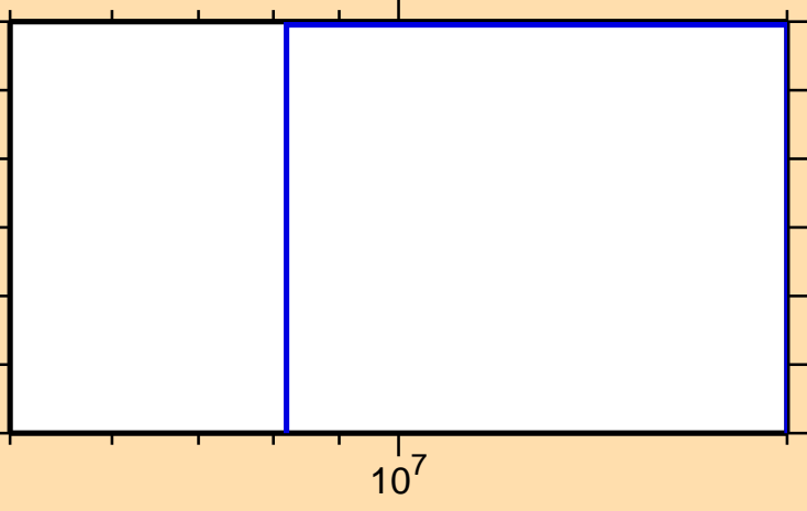
\sigma vs. E for ^{132}\text{Sm}(n,2n)
