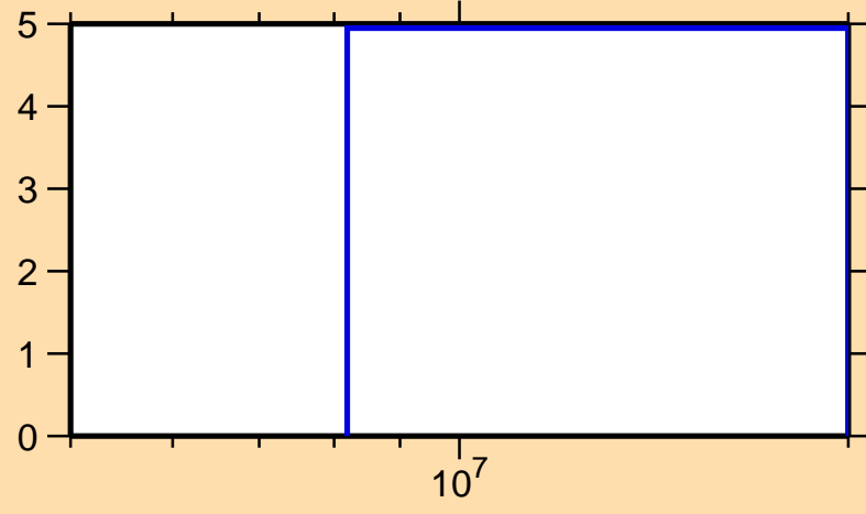
\Delta\sigma/\sigma vs. E for ^{132}\text{Sm}(n,\text{tot.})
