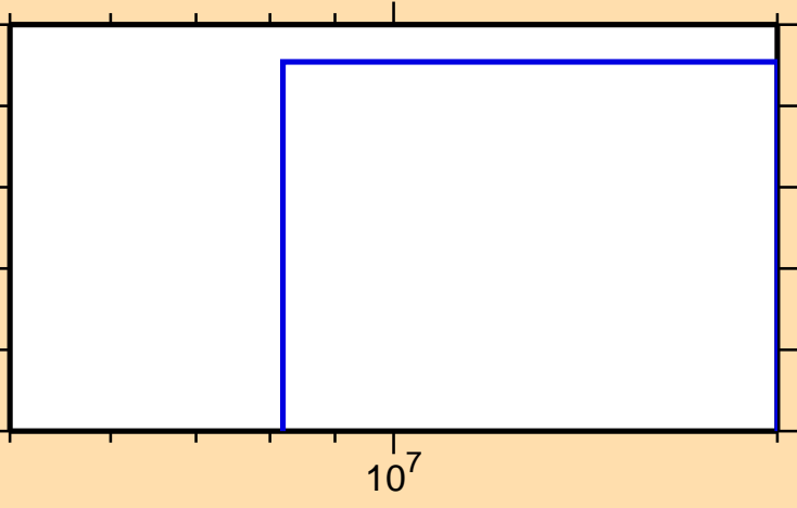
\sigma vs. E for ^{133}\text{Sm} (mt 34)
