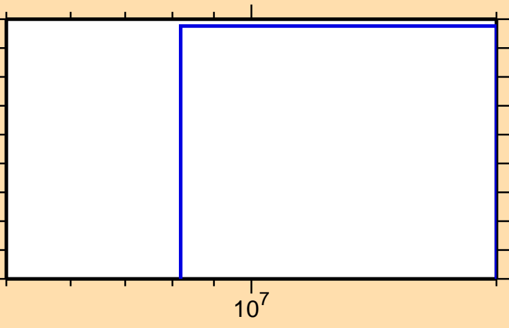
\sigma vs. E for ^{133}\text{Sm}(n,2np)
