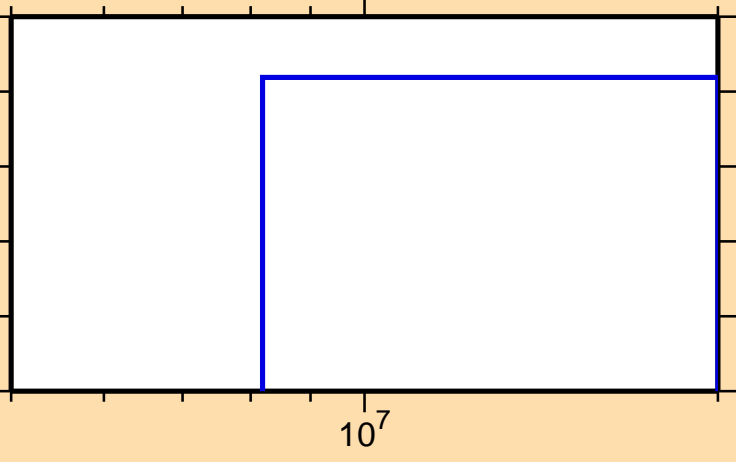
\sigma vs. E for ^{133}\text{Sm}(\text{mt117})
