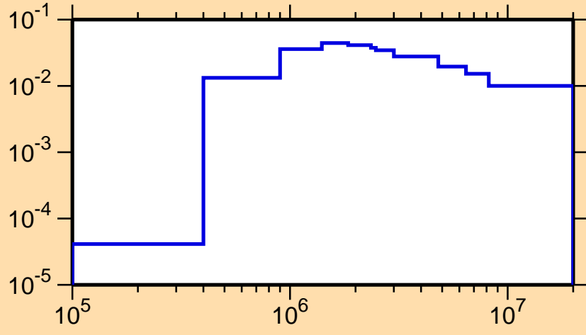
\sigma vs. E for ^{133}\text{Sm}(n,n_3)
