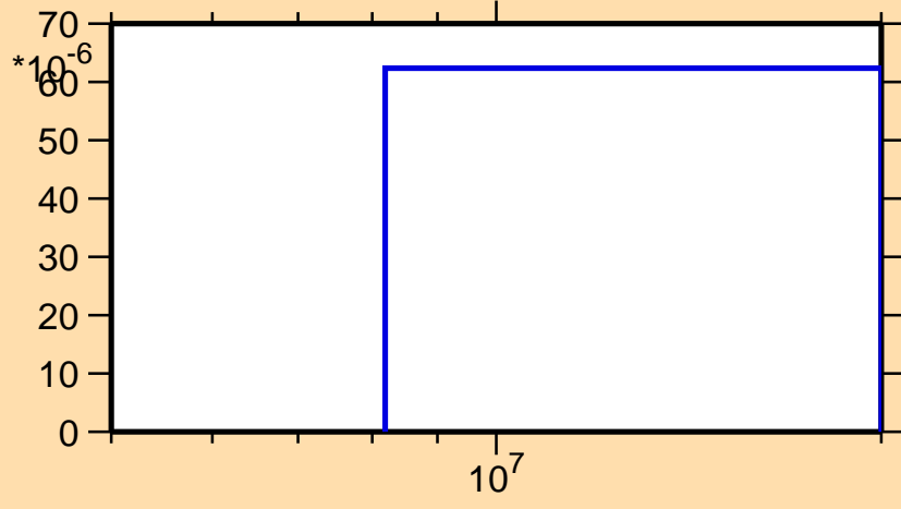
\sigma vs. E for ^{133}\text{Sm}(n,\text{pt})
