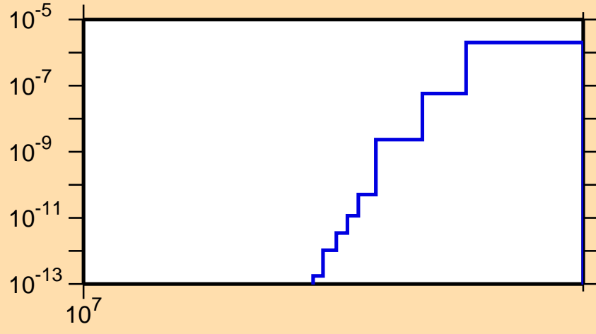
\sigma vs. E for ^{134}\text{Sm}(n,pt)
