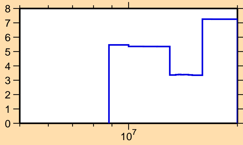
\Delta\sigma/\sigma vs. E for ^{135}\text{Sm}(n,\text{el.})
