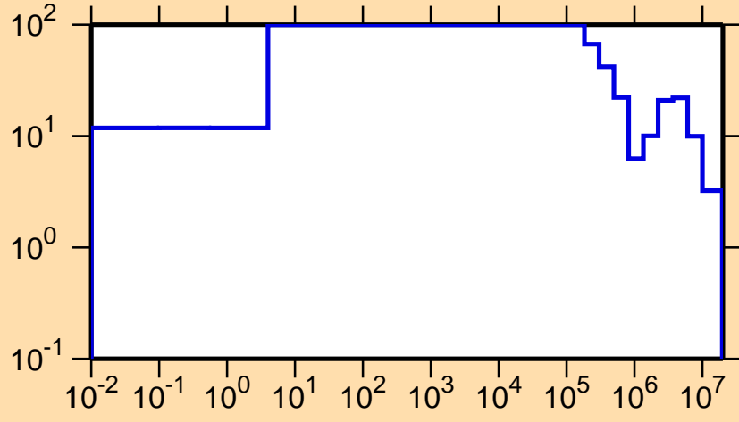
\Delta\sigma/\sigma vs. E for ^{135}\text{Sm}(n,el.)
