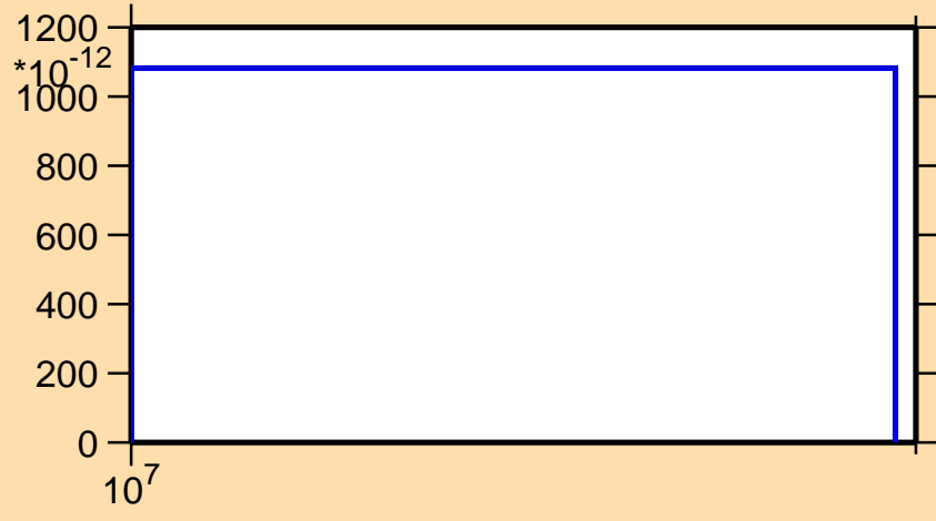
\sigma vs. E for ^{135}\text{Sm} (mt 34)
