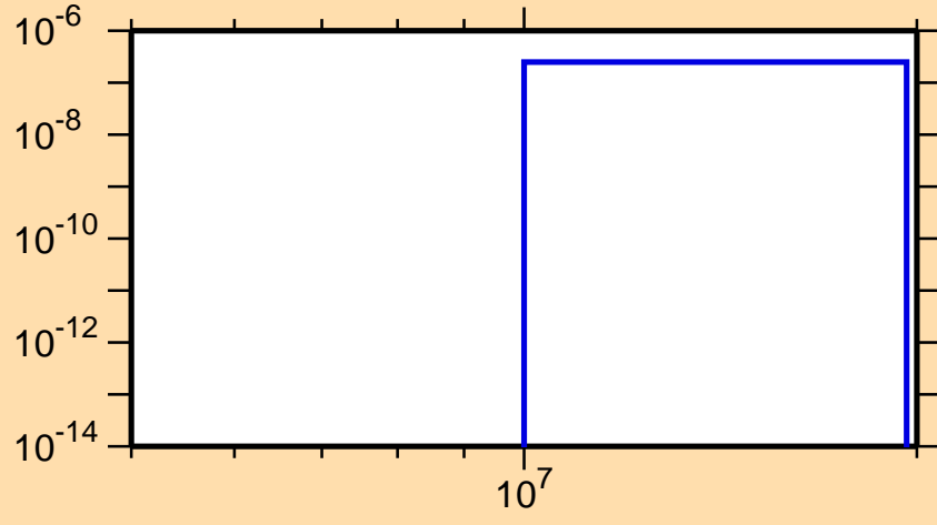
\sigma vs. E for ^{135}\text{Sm} (mt 45)
