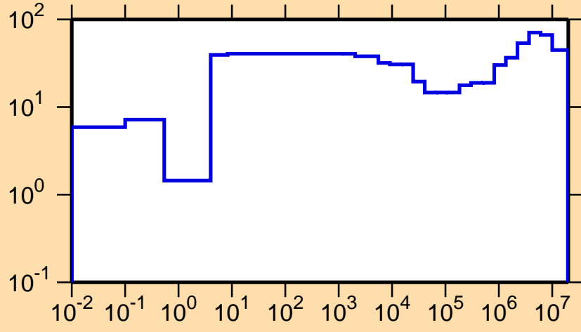
\Delta\sigma/\sigma vs. E for ^{135}\text{Sm}(n,\gamma)
