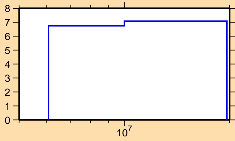
\Delta\sigma/\sigma vs. E for ^{135}\text{Sm}(n,\text{nonel.})
