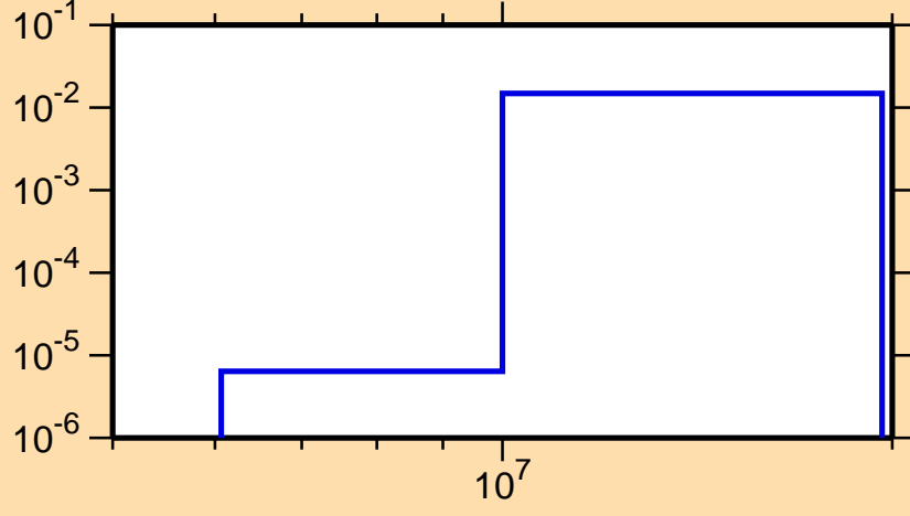
\sigma vs. E for ^{135}\text{Sm}(n,2n)
