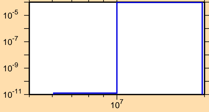
\sigma vs. E for ^{135}\text{Sm}(n,\text{pd})
