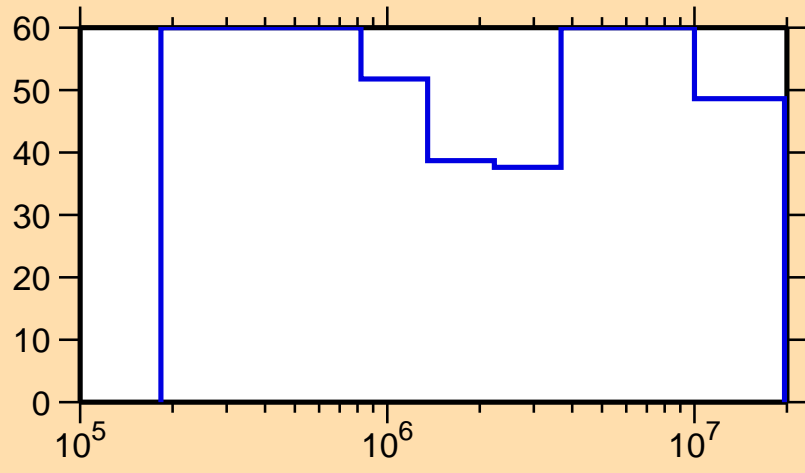
\Delta\sigma/\sigma vs. E for ^{135}\text{Sm}(n,n_1)
