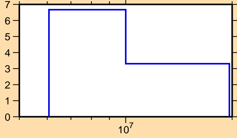
\Delta\sigma/\sigma vs. E for ^{135}\text{Sm}(n,\text{tot.})
