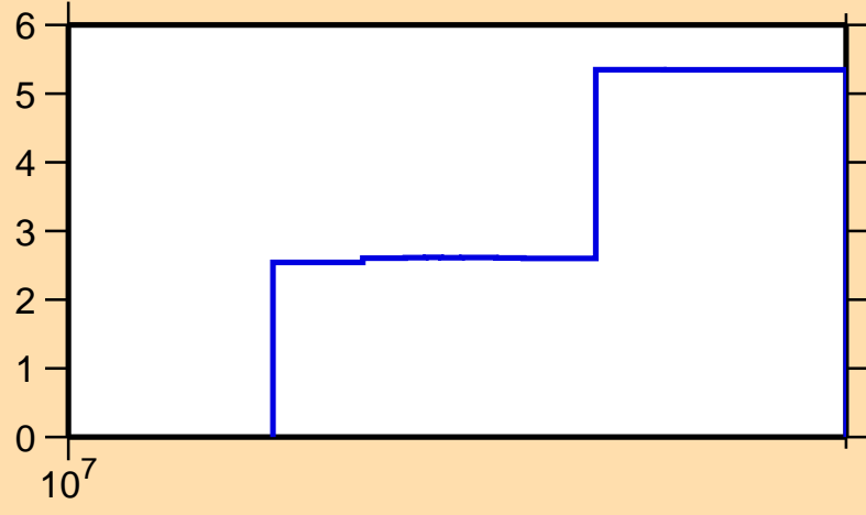
\Delta\sigma/\sigma vs. E for ^{136}\text{Sm}(n,\text{tot.})
