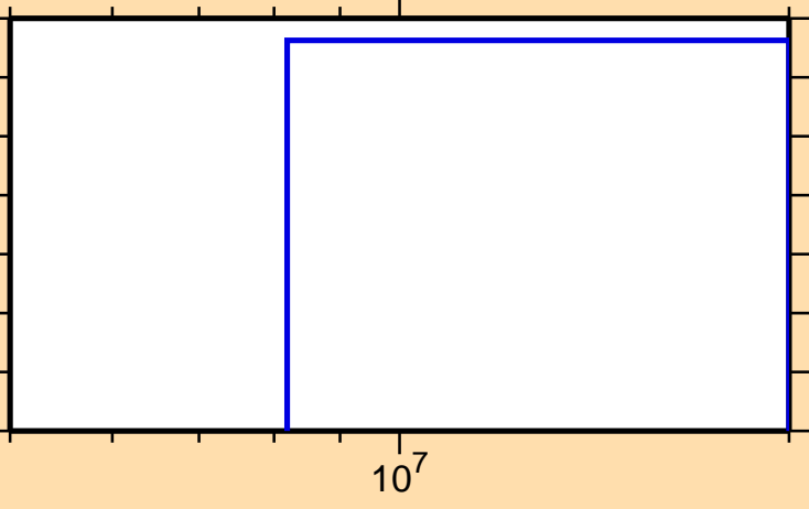
\sigma vs. E for ^{136}\text{Sm}(\text{mt117})
