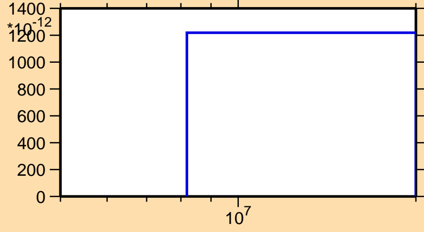
\sigma vs. E for ^{136}\text{Sm}(n,pt)
