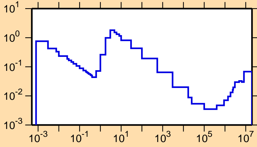
\sigma vs. E for ^{136}\text{Sm}(n,\alpha)
