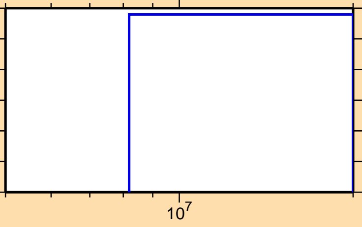
\sigma vs. E for ^{136}\text{Sm}(n,\text{nd})
