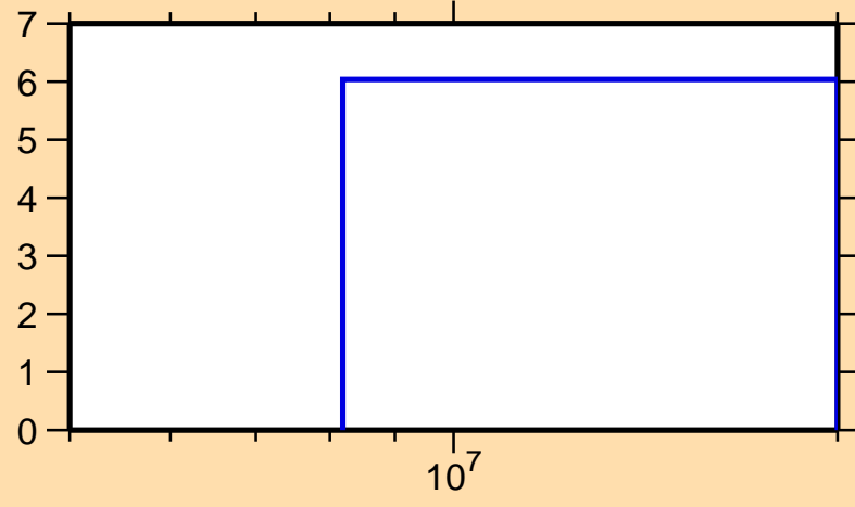
\Delta\sigma/\sigma vs. E for ^{136}\text{Sm}(n,\text{nonel.})
