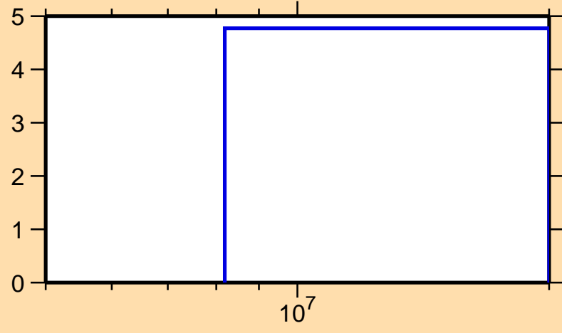
\Delta\sigma/\sigma vs. E for ^{136}\text{Sm}(n,\text{el.})
