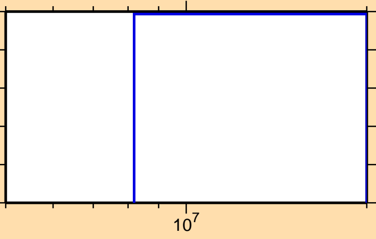
\sigma vs. E for ^{136}\text{Sm} (mt 45)
