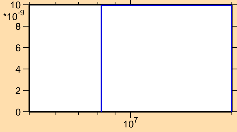
\sigma vs. E for ^{136}\text{Sm}(n,2np)
