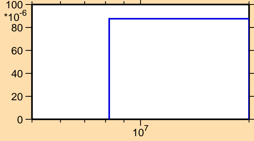
\sigma vs. E for ^{136}\text{Sm}(n,\text{pd})
