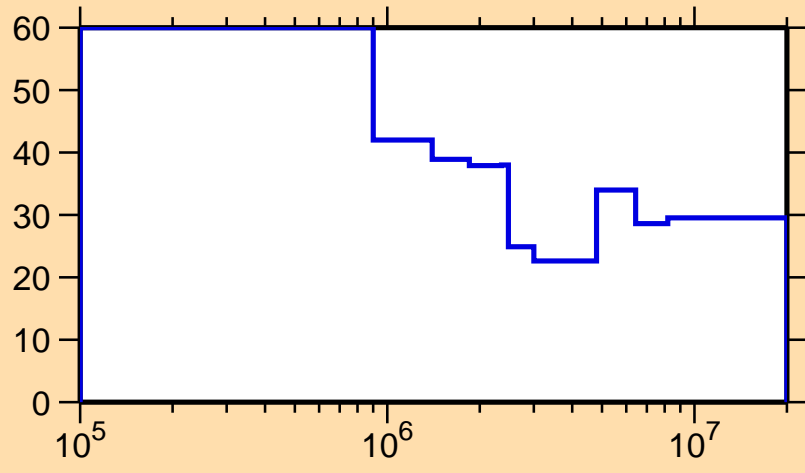
\Delta\sigma/\sigma vs. E for ^{136}\text{Sm}(n,\text{inel.})
