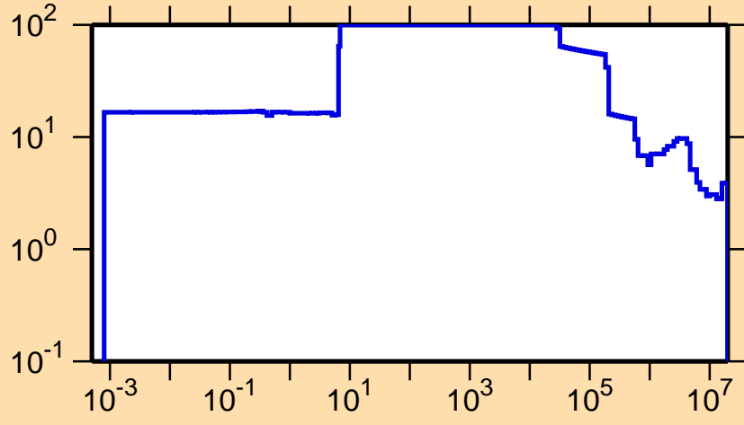
\Delta\sigma/\sigma vs. E for ^{137}\text{Sm}(n,el.)
