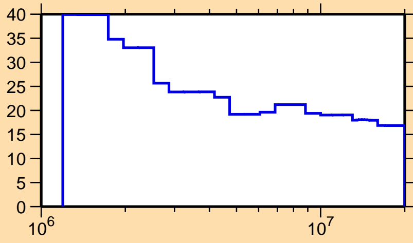
\Delta\sigma/\sigma vs. E for ^{137}\text{Sm}(n,n_1)
