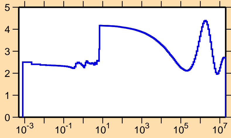
\sigma vs. E for ^{137}\text{Sm}(n,\text{el.})
