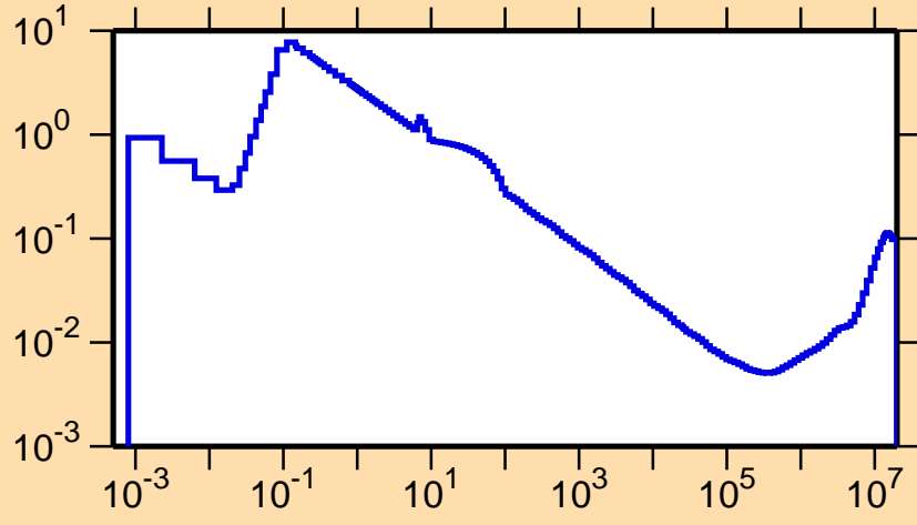
\sigma vs. E for ^{137}\text{Sm}(n,\alpha)
