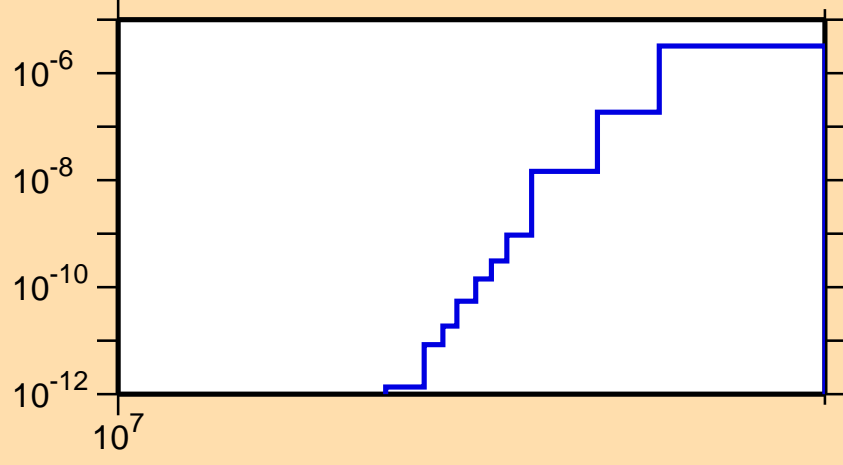
\sigma vs. E for ^{137}\text{Sm}(n,2n\alpha)
