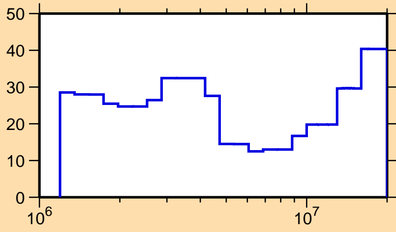
\Delta\sigma/\sigma vs. E for ^{137}\text{Sm}(n,n\text{cont.})
