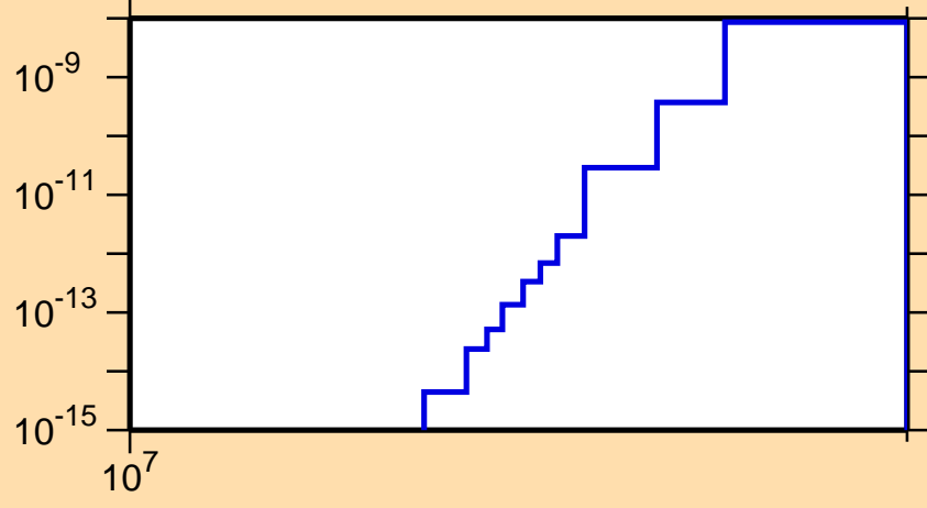
\sigma vs. E for ^{137}\text{Sm} (mt 34)
