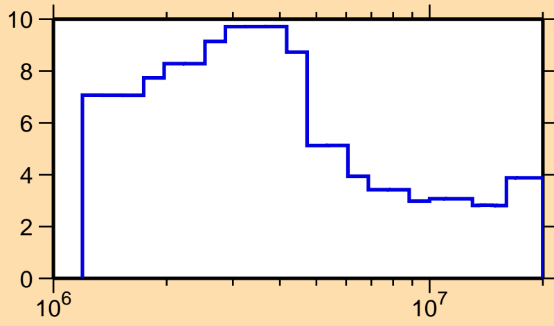
\Delta\sigma/\sigma vs. E for ^{137}\text{Sm}(n, el.)
