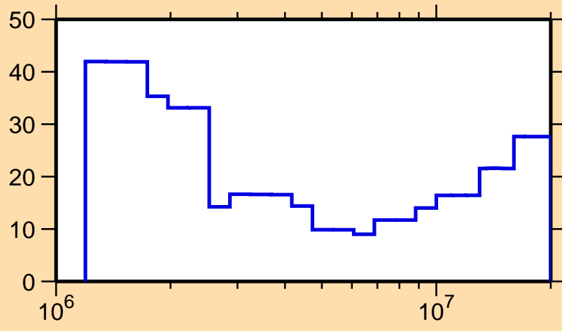
\Delta\sigma/\sigma vs. E for ^{137}\text{Sm}(n,\text{inel.})
