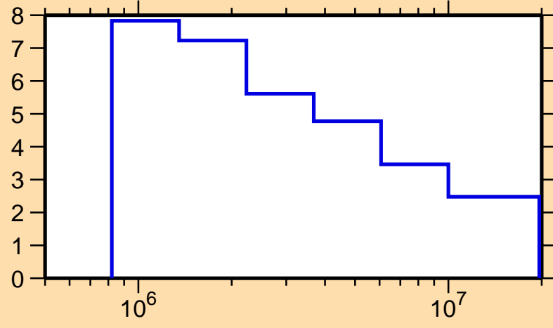
\Delta\sigma/\sigma vs. E for ^{137}\text{Sm}(n, \text{tot.})
