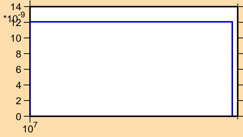
\sigma vs. E for ^{137}\text{Sm}(n,\text{nd})
