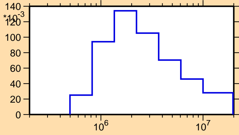
\sigma vs. E for ^{137}\text{Sm}(n,n_4)
