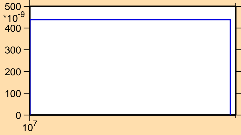
\sigma vs. E for ^{137}\text{Sm}(n,pt)
