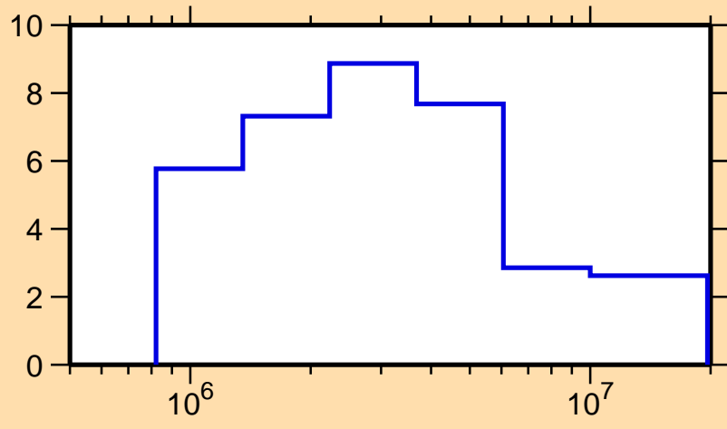
\Delta\sigma/\sigma vs. E for ^{137}\text{Sm}(n,\text{el.})
