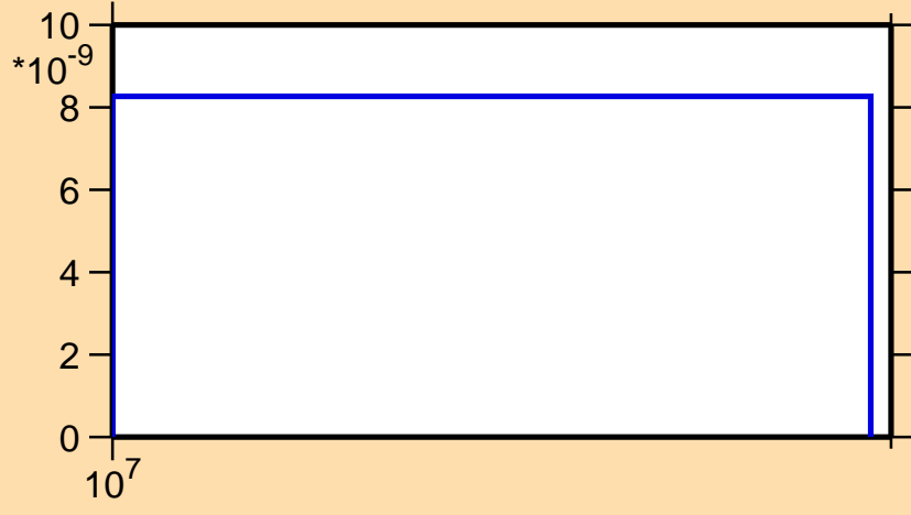
\sigma vs. E for ^{137}\text{Sm} (mt 45)
