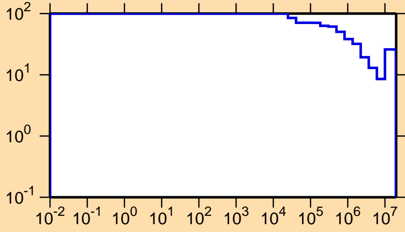
\Delta\sigma/\sigma vs. E for ^{137}\text{Sm}(n,p)
