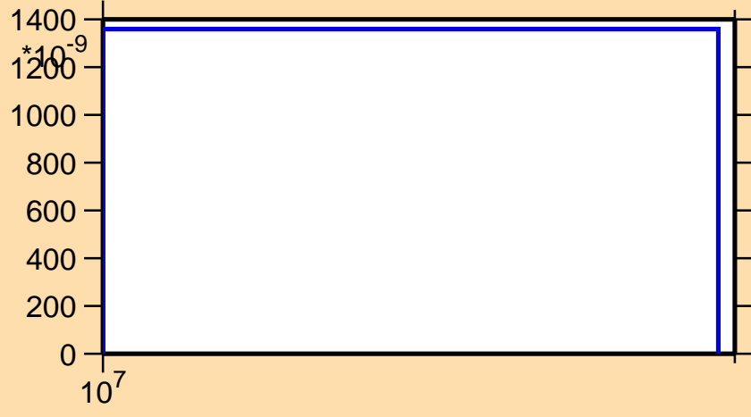
\sigma vs. E for ^{137}\text{Sm}(n,2np)
