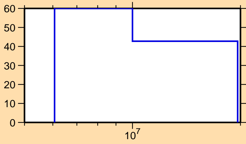
\Delta\sigma/\sigma vs. E for ^{137}\text{Sm}(n,2n)
