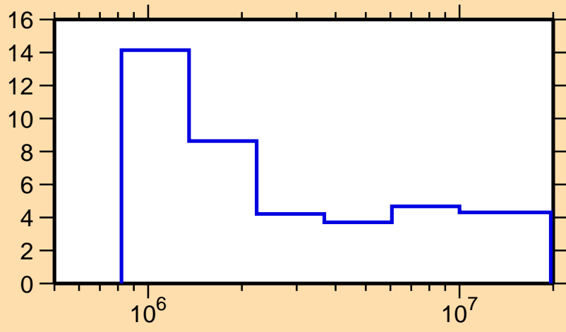
\Delta\sigma/\sigma vs. E for ^{137}\text{Sm}(n, \text{nonel.})
