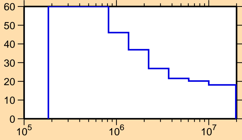
\Delta\sigma/\sigma vs. E for ^{137}\text{Sm}(n,n_1)
