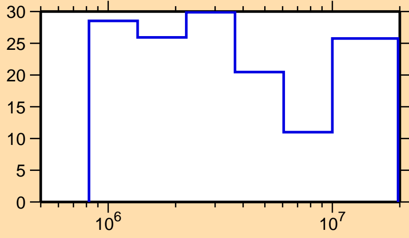
\Delta\sigma/\sigma vs. E for ^{137}\text{Sm}(n,n\text{cont.})
