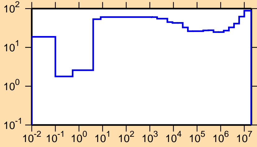
\Delta\sigma/\sigma vs. E for ^{137}\text{Sm}(n,\gamma)
