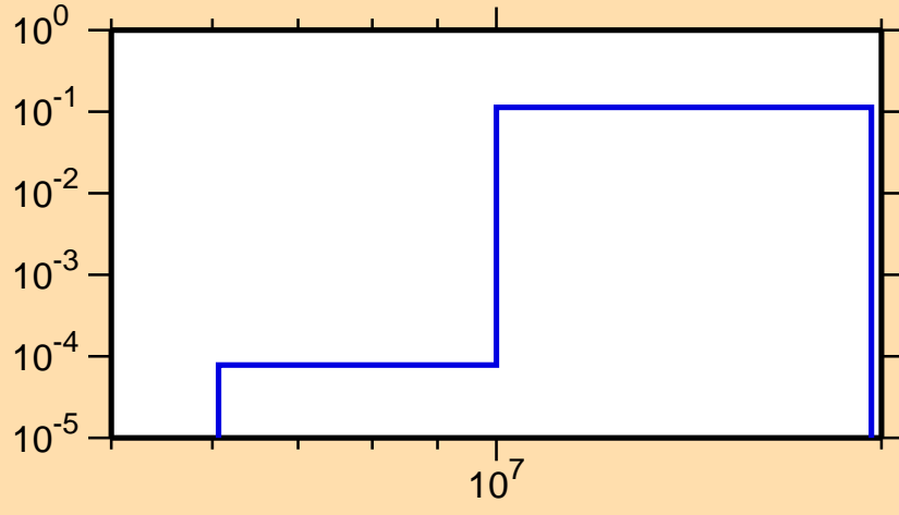
\sigma vs. E for ^{137}\text{Sm}(n,2n)
