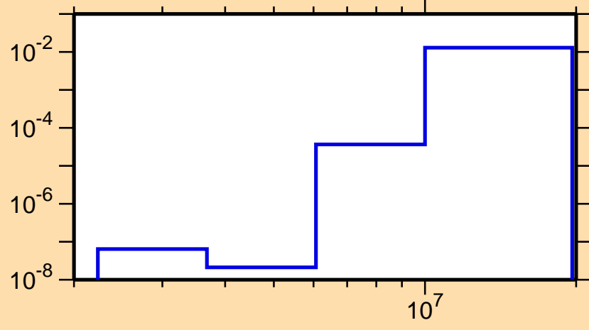
\sigma vs. E for ^{137}\text{Sm}(n,n\alpha)
