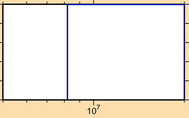
\sigma vs. E for ^{137}\text{Sm}(n,\text{pd})
