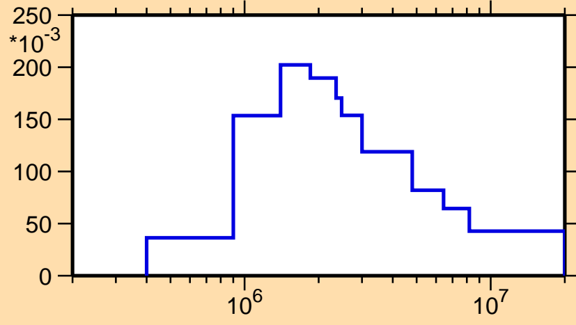
\sigma vs. E for ^{137}\text{Sm}(n,n_3)
