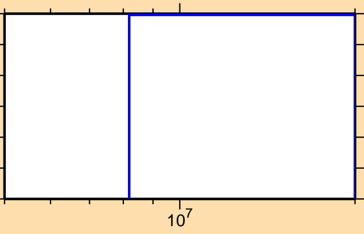
\sigma vs. E for ^{137}\text{Sm}(n,2np)
